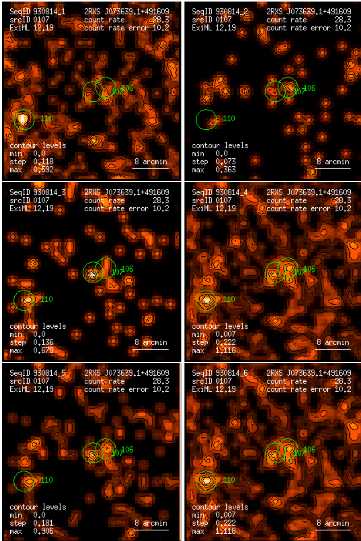
Figure 107: RASS 930814: detection 0107: band rate images, Gaussian filter: (1) PSPC channels 11 – 41, (2) 52 – 90, (3) 91 – 201, (4) 11 – 235, (5) 52 – 201, (6) 11 – 201. Broad band rates in counts/ks. Band rate contour levels in counts/ks/arcmin 2 .
