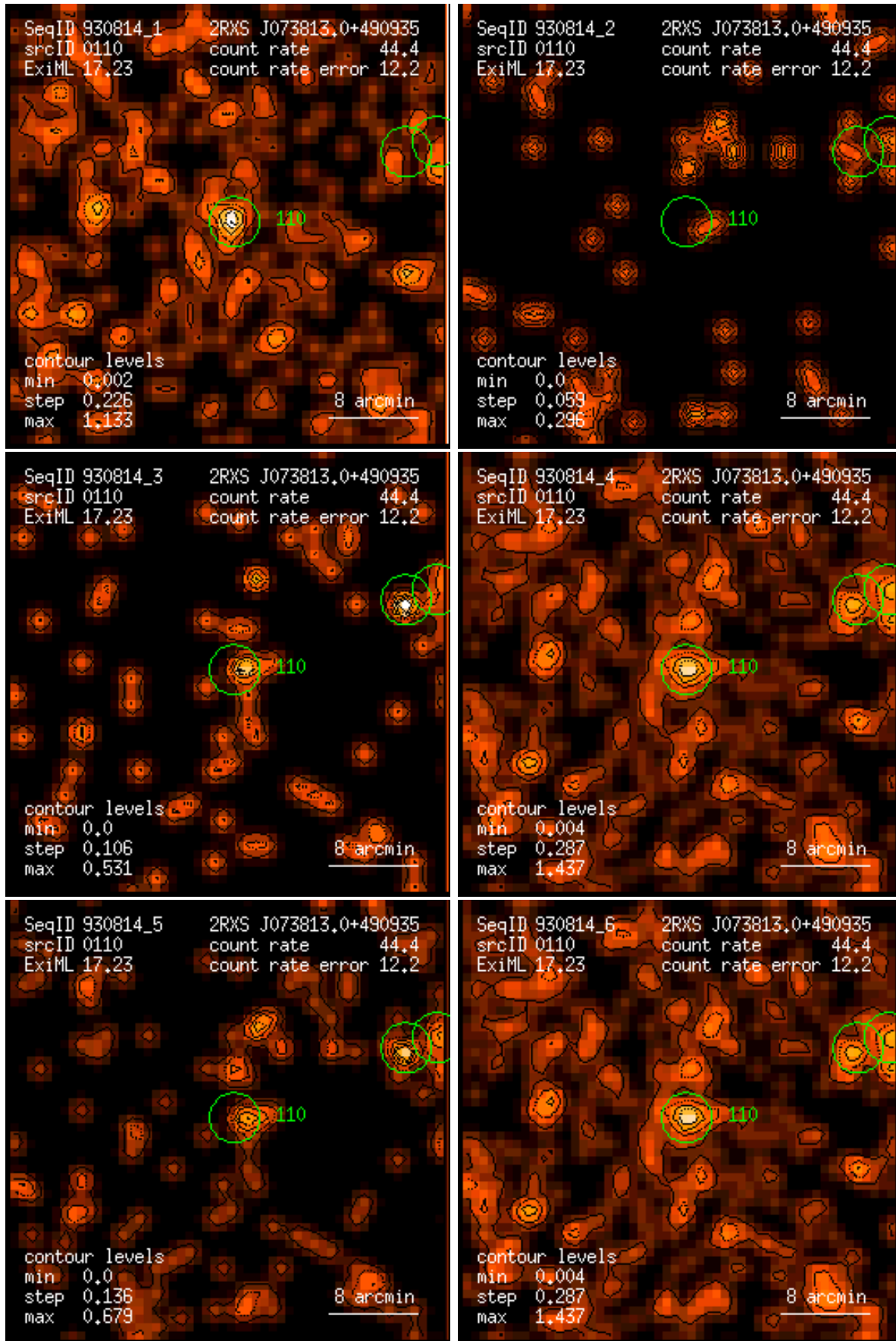
Figure 110: RASS 930814: detection 0110: band rate images, Gaussian filter: (1) PSPC channels 11 – 41, (2) 52 – 90, (3) 91 – 201, (4) 11 – 235, (5) 52 – 201, (6) 11 – 201. Broad band rates in counts/ks. Band rate contour levels in counts/ks/arcmin 2 .
