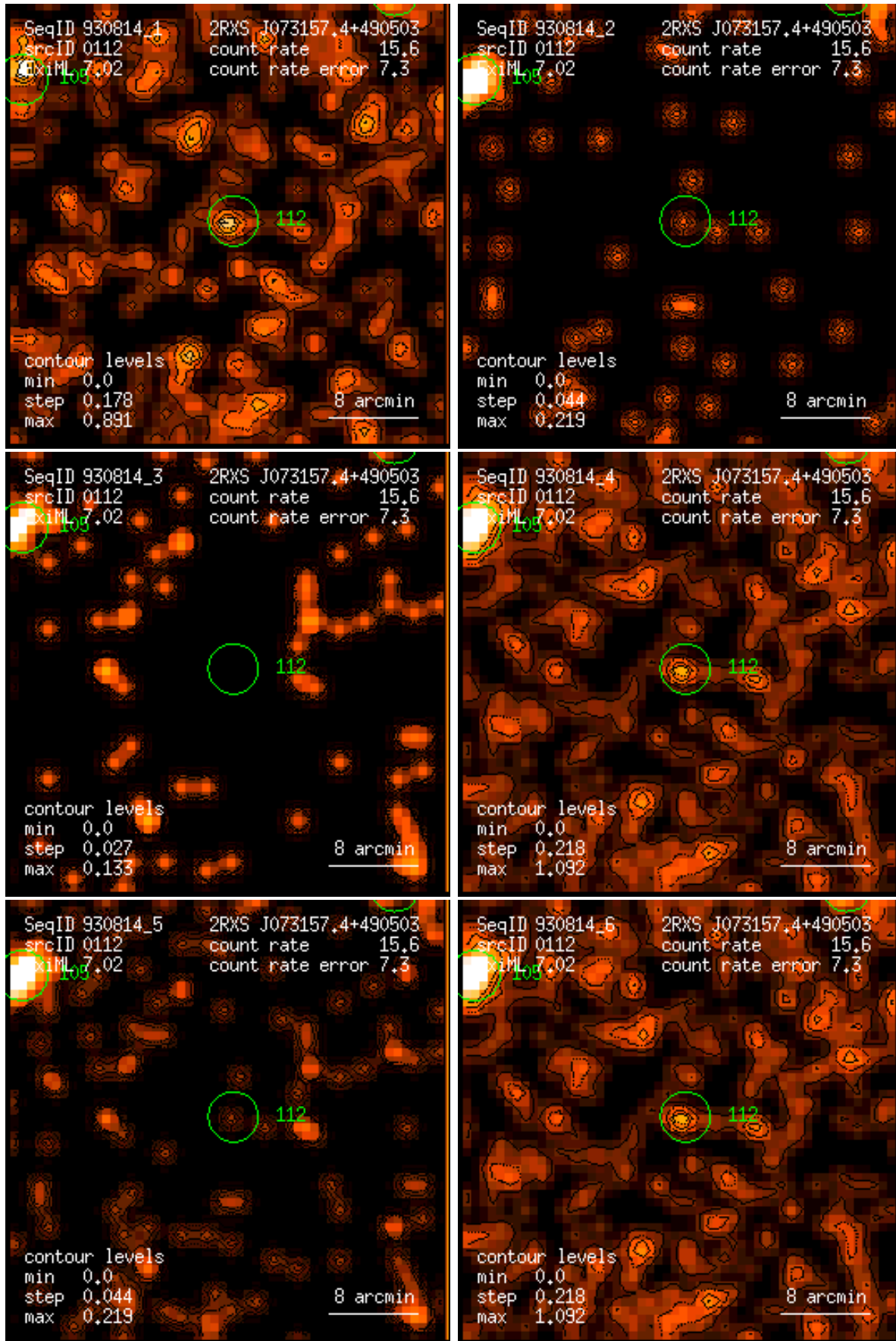
Figure 112: RASS 930814: detection 0112: band rate images, Gaussian filter: (1) PSPC channels 11 – 41, (2) 52 – 90, (3) 91 – 201, (4) 11 – 235, (5) 52 – 201, (6) 11 – 201. Broad band rates in counts/ks. Band rate contour levels in counts/ks/arcmin 2 .
