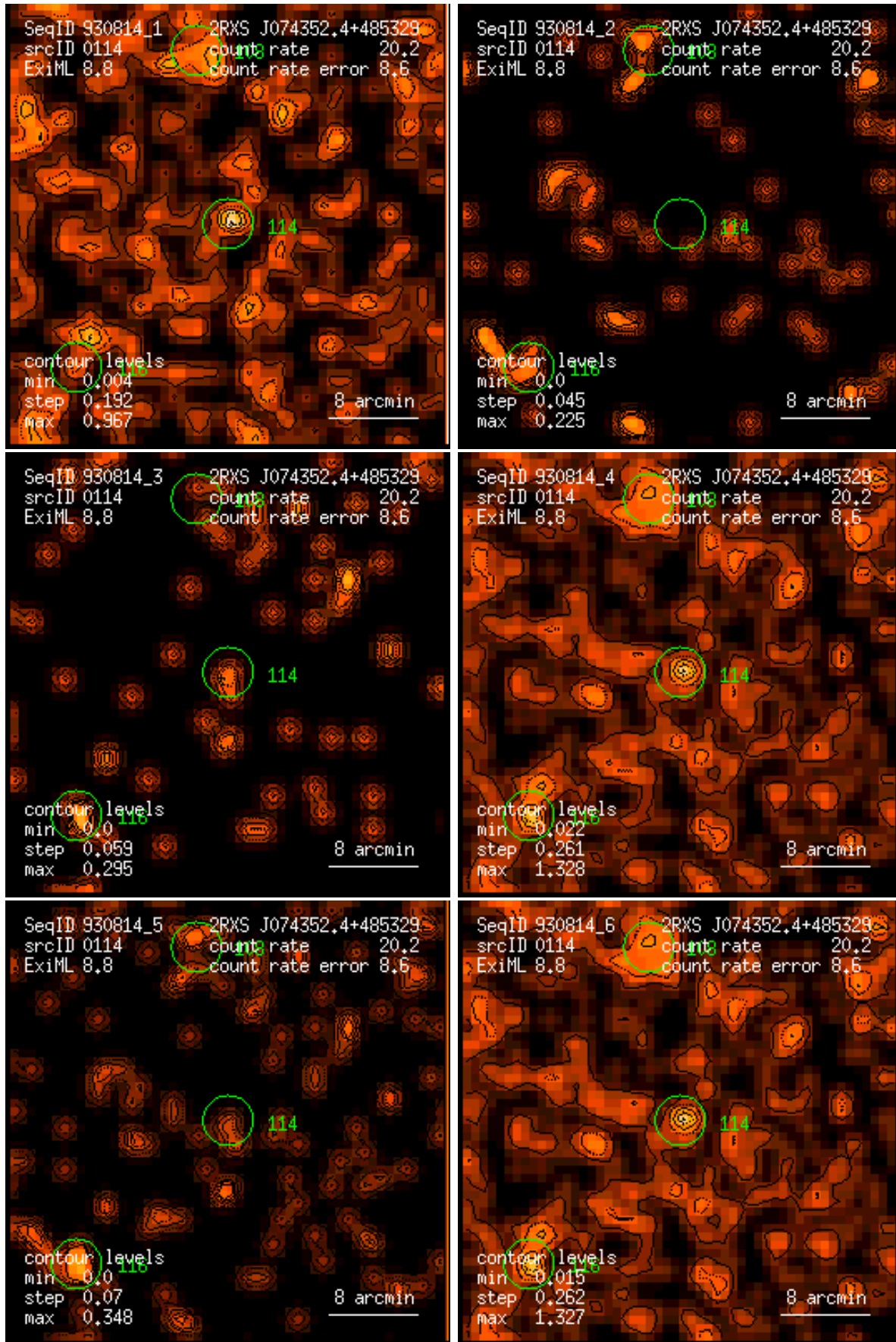
Figure 114: RASS 930814: detection 0114: band rate images, Gaussian filter: (1) PSPC channels 11 – 41, (2) 52 – 90, (3) 91 – 201, (4) 11 – 235, (5) 52 – 201, (6) 11 – 201. Broad band rates in counts/ks. Band rate contour levels in counts/ks/arcmin 2 .
