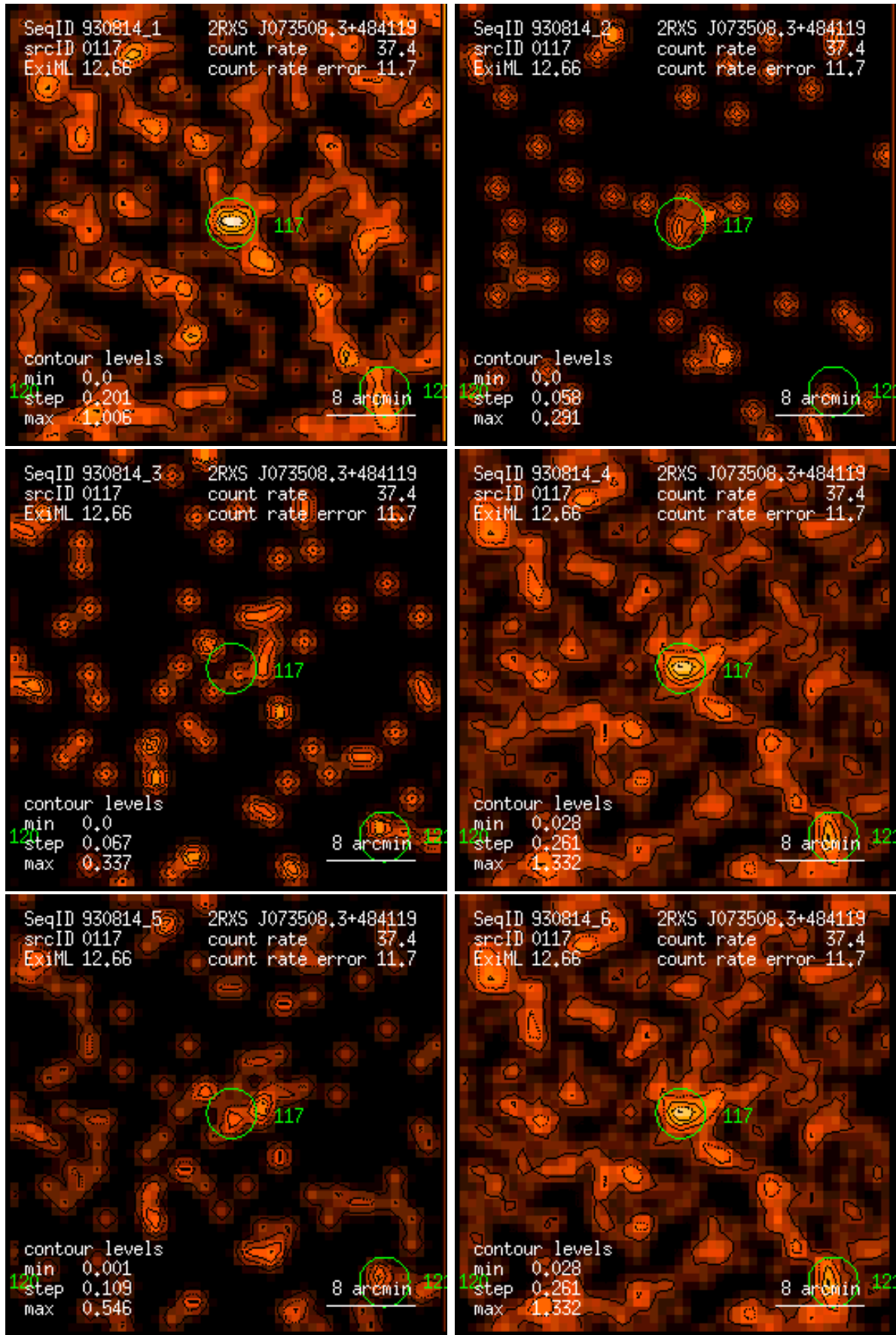
Figure 117: RASS 930814: detection 0117: band rate images, Gaussian filter: (1) PSPC channels 11 – 41, (2) 52 – 90, (3) 91 – 201, (4) 11 – 235, (5) 52 – 201, (6) 11 – 201. Broad band rates in counts/ks. Band rate contour levels in counts/ks/arcmin 2 .
