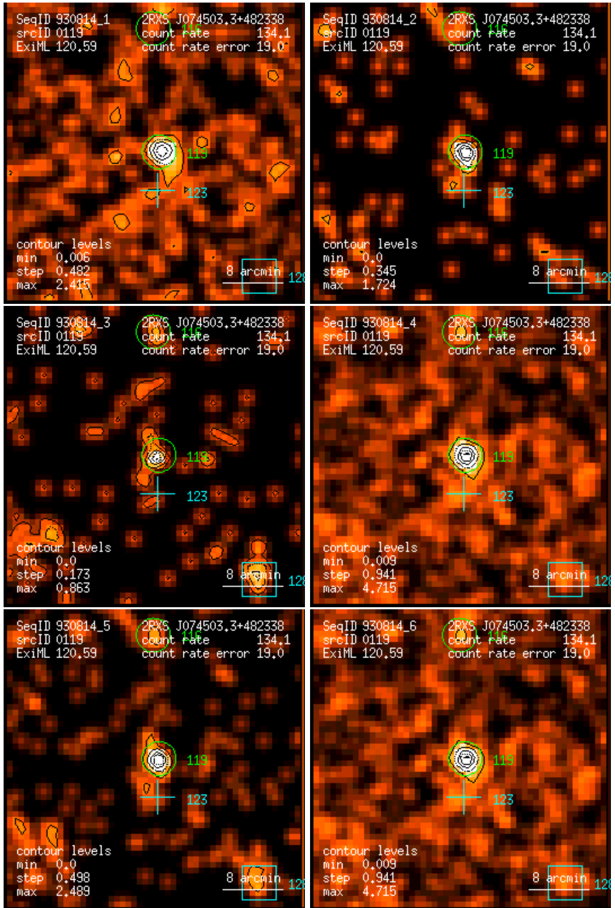
Figure 119: RASS 930814: detection 0119: band rate images, Gaussian filter: (1) PSPC channels 11 – 41, (2) 52 – 90, (3) 91 – 201, (4) 11 – 235, (5) 52 – 201, (6) 11 – 201. Broad band rates in counts/ks. Band rate contour levels in counts/ks/arcmin 2 .
