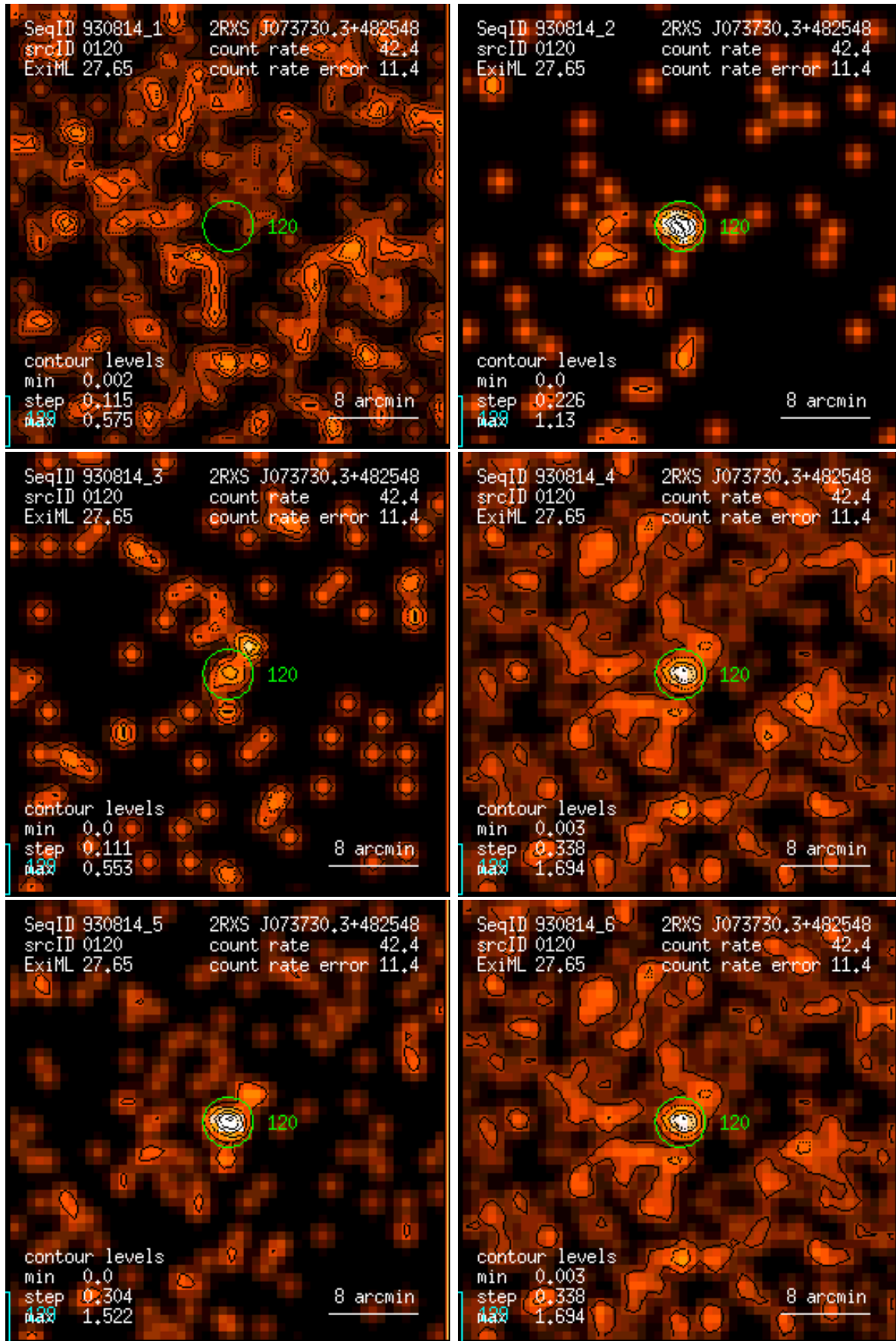
Figure 120: RASS 930814: detection 0120: band rate images, Gaussian filter: (1) PSPC channels 11 – 41, (2) 52 – 90, (3) 91 – 201, (4) 11 – 235, (5) 52 – 201, (6) 11 – 201. Broad band rates in counts/ks. Band rate contour levels in counts/ks/arcmin 2 .
