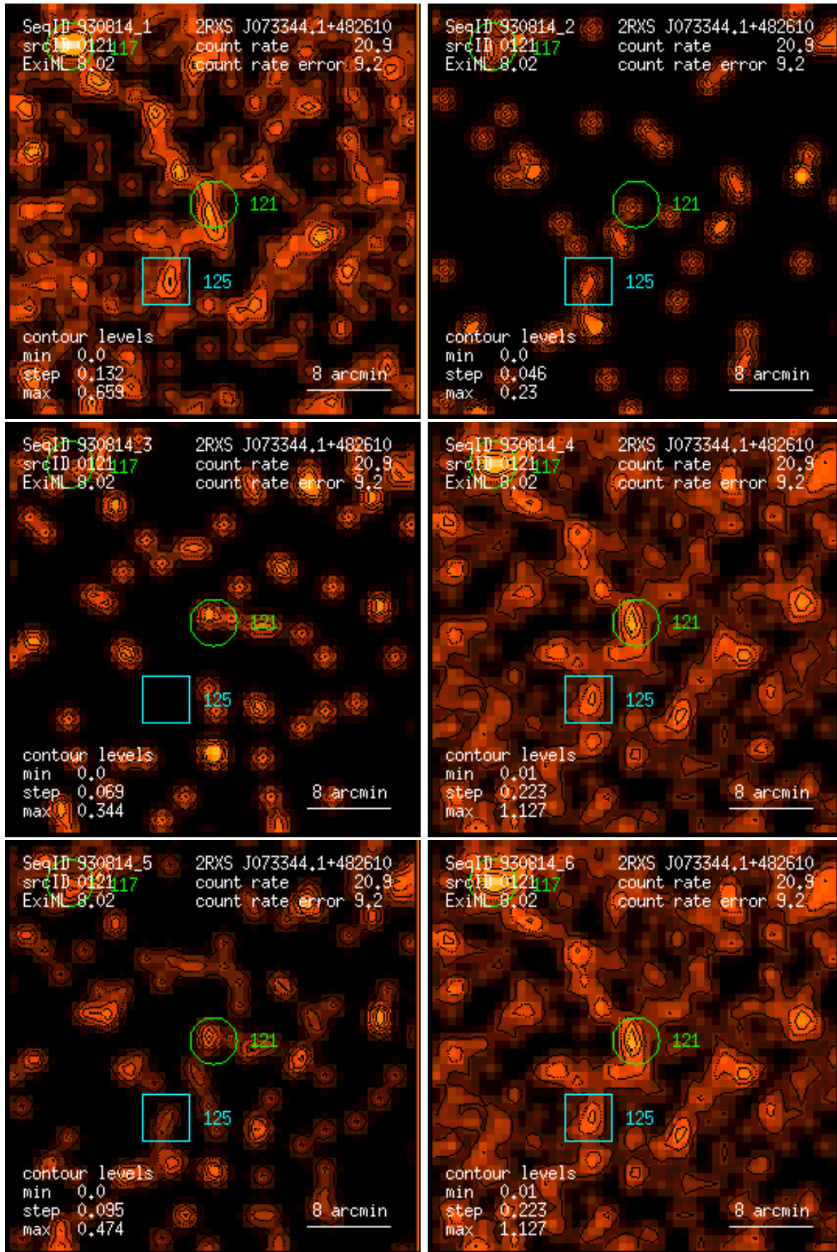
Figure 121: RASS 930814: detection 0121: band rate images, Gaussian filter: (1) PSPC channels 11 – 41, (2) 52 – 90, (3) 91 – 201, (4) 11 – 235, (5) 52 – 201, (6) 11 – 201. Broad band rates in counts/ks. Band rate contour levels in counts/ks/arcmin 2 .
