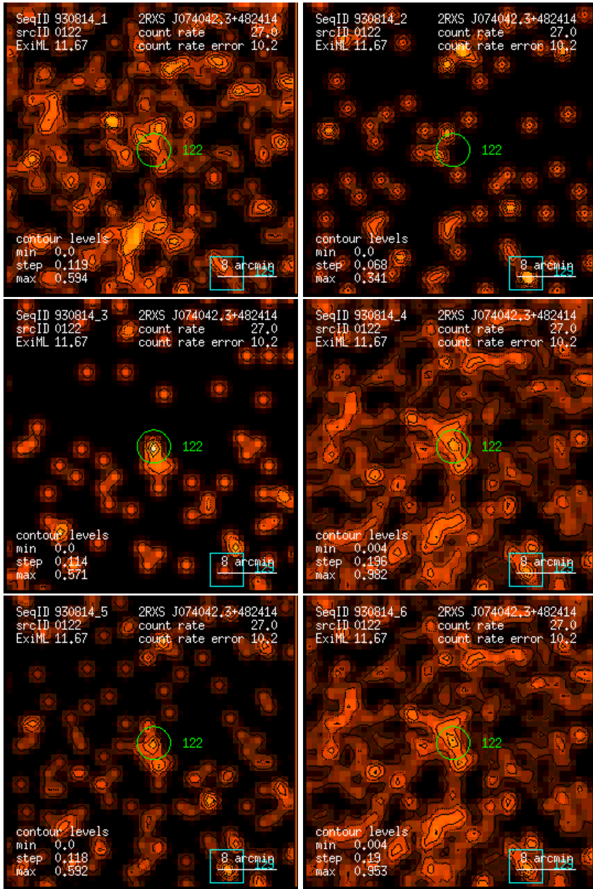
Figure 122: RASS 930814: detection 0122: band rate images, Gaussian filter: (1) PSPC channels 11 – 41, (2) 52 – 90, (3) 91 – 201, (4) 11 – 235, (5) 52 – 201, (6) 11 – 201. Broad band rates in counts/ks. Band rate contour levels in counts/ks/arcmin 2 .
