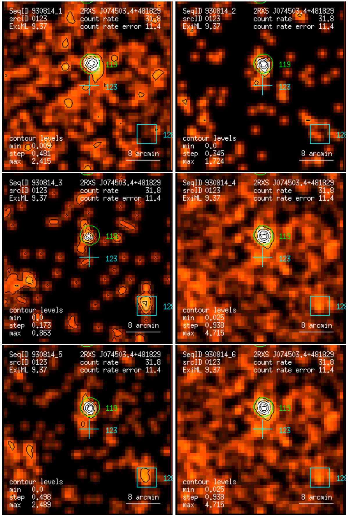
Figure 123: RASS 930814: detection 0123: band rate images, Gaussian filter: (1) PSPC channels 11 – 41, (2) 52 – 90, (3) 91 – 201, (4) 11 – 235, (5) 52 – 201, (6) 11 – 201. Broad band rates in counts/ks. Band rate contour levels in counts/ks/arcmin 2 .
