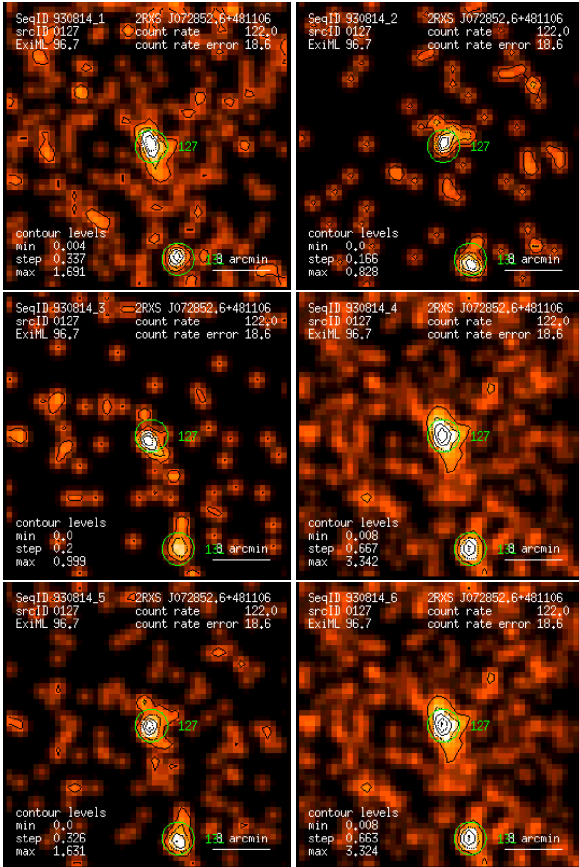
Figure 127: RASS 930814: detection 0127: band rate images, Gaussian filter: (1) PSPC channels 11 – 41, (2) 52 – 90, (3) 91 – 201, (4) 11 – 235, (5) 52 – 201, (6) 11 – 201. Broad band rates in counts/ks. Band rate contour levels in counts/ks/arcmin 2 .
