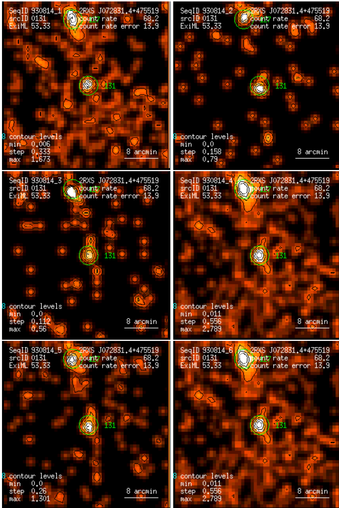
Figure 131: RASS 930814: detection 0131: band rate images, Gaussian filter: (1) PSPC channels 11 – 41, (2) 52 – 90, (3) 91 – 201, (4) 11 – 235, (5) 52 – 201, (6) 11 – 201. Broad band rates in counts/ks. Band rate contour levels in counts/ks/arcmin 2 .
