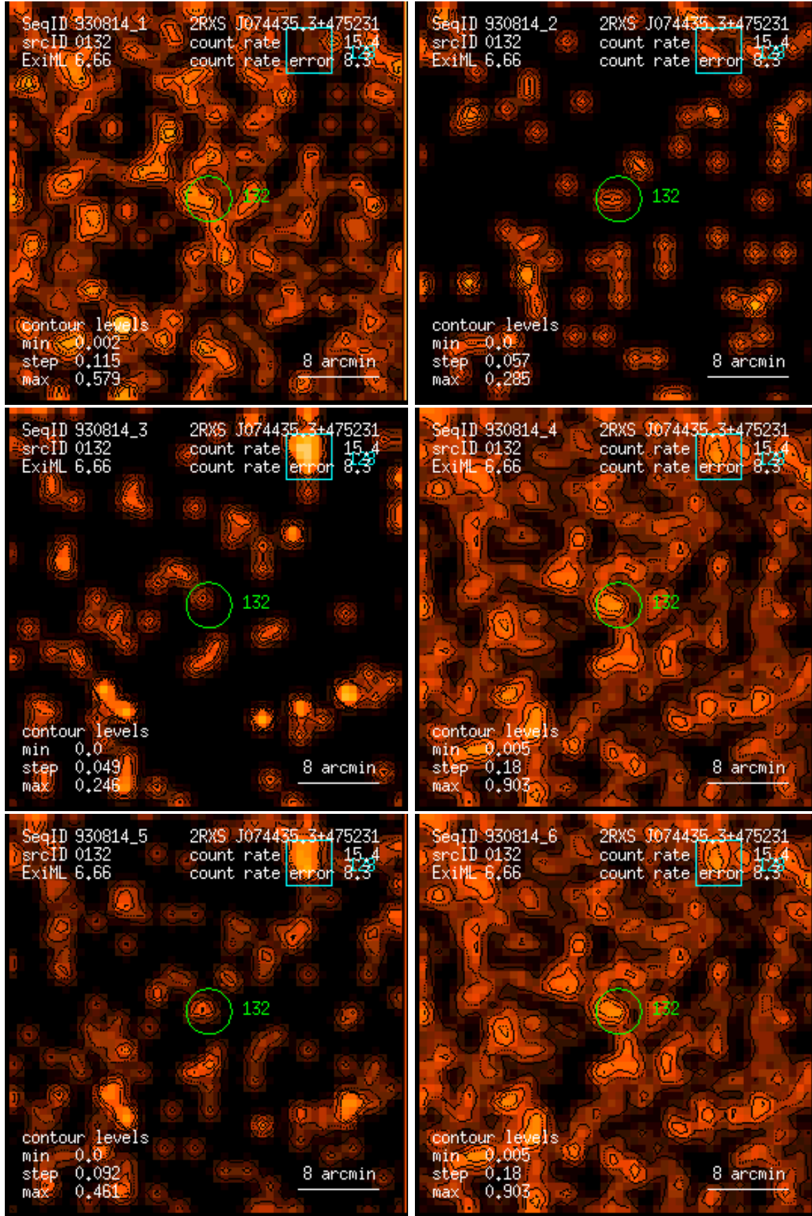
Figure 132: RASS 930814: detection 0132: band rate images, Gaussian filter: (1) PSPC channels 11 – 41, (2) 52 – 90, (3) 91 – 201, (4) 11 – 235, (5) 52 – 201, (6) 11 – 201. Broad band rates in counts/ks. Band rate contour levels in counts/ks/arcmin 2 .
