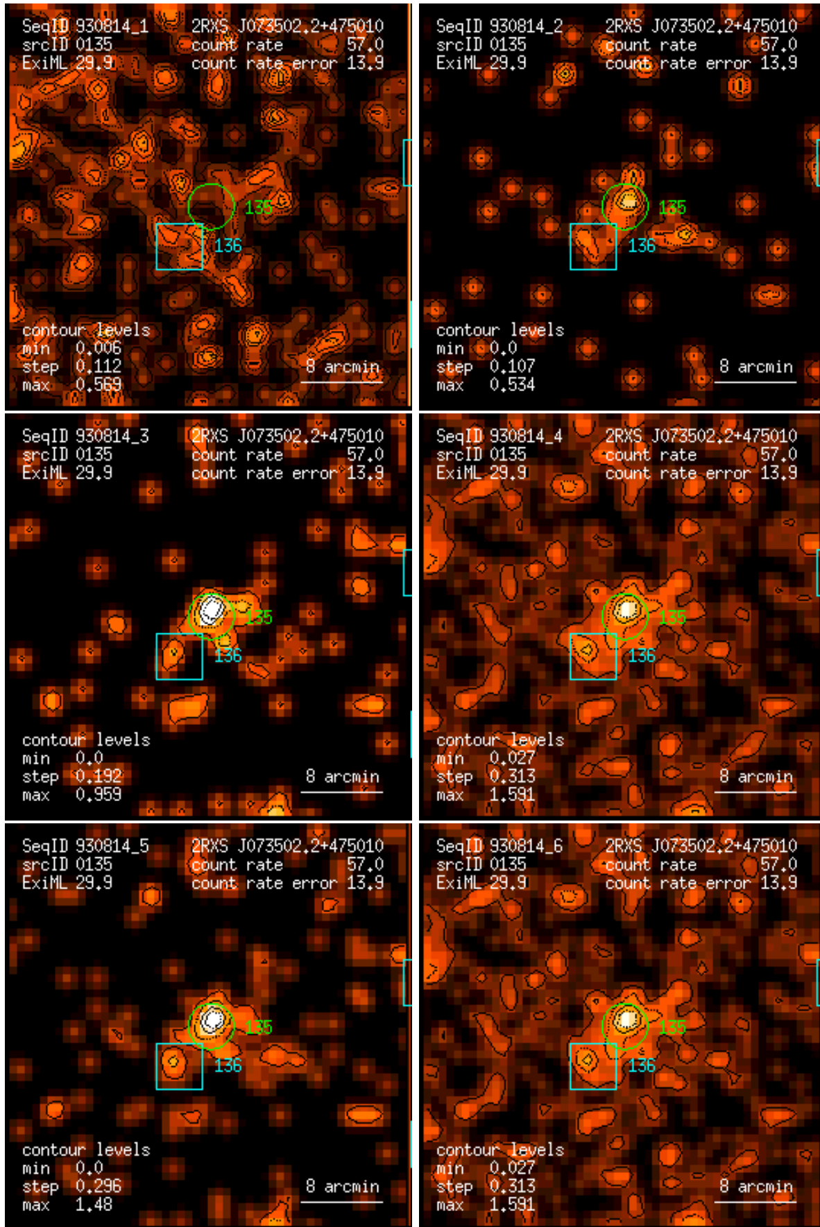
Figure 135: RASS 930814: detection 0135: band rate images, Gaussian filter: (1) PSPC channels 11 – 41, (2) 52 – 90, (3) 91 – 201, (4) 11 – 235, (5) 52 – 201, (6) 11 – 201. Broad band rates in counts/ks. Band rate contour levels in counts/ks/arcmin 2 .
