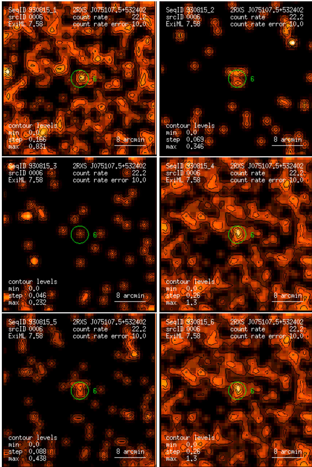
Figure 6: RASS 930815: detection 0006: band rate images, Gaussian filter: (1) PSPC channels 11 – 41, (2) 52 – 90, (3) 91 – 201, (4) 11 – 235, (5) 52 – 201, (6) 11 – 201. Broad band rates in counts/ks. Band rate contour levels in counts/ks/arcmin 2 .
