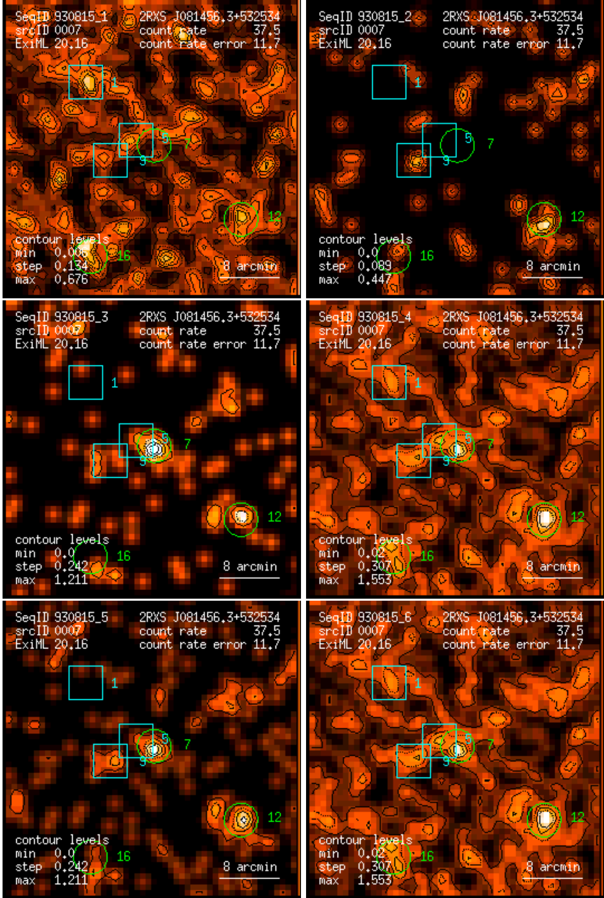
Figure 7: RASS 930815: detection 0007: band rate images, Gaussian filter: (1) PSPC channels 11 – 41, (2) 52 – 90, (3) 91 – 201, (4) 11 – 235, (5) 52 – 201, (6) 11 – 201. Broad band rates in counts/ks. Band rate contour levels in counts/ks/arcmin 2 .
