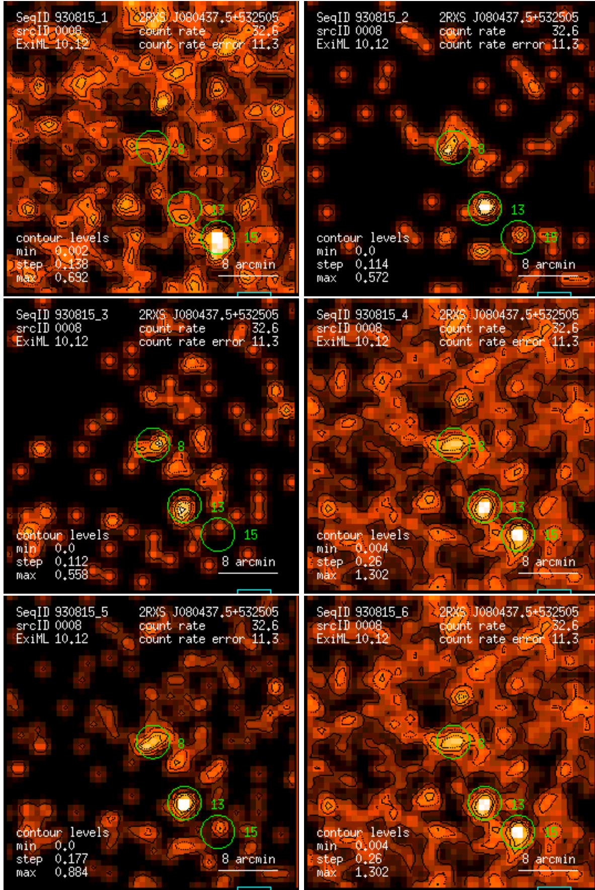
Figure 8: RASS 930815: detection 0008: band rate images, Gaussian filter: (1) PSPC channels 11 – 41, (2) 52 – 90, (3) 91 – 201, (4) 11 – 235, (5) 52 – 201, (6) 11 – 201. Broad band rates in counts/ks. Band rate contour levels in counts/ks/arcmin 2 .
