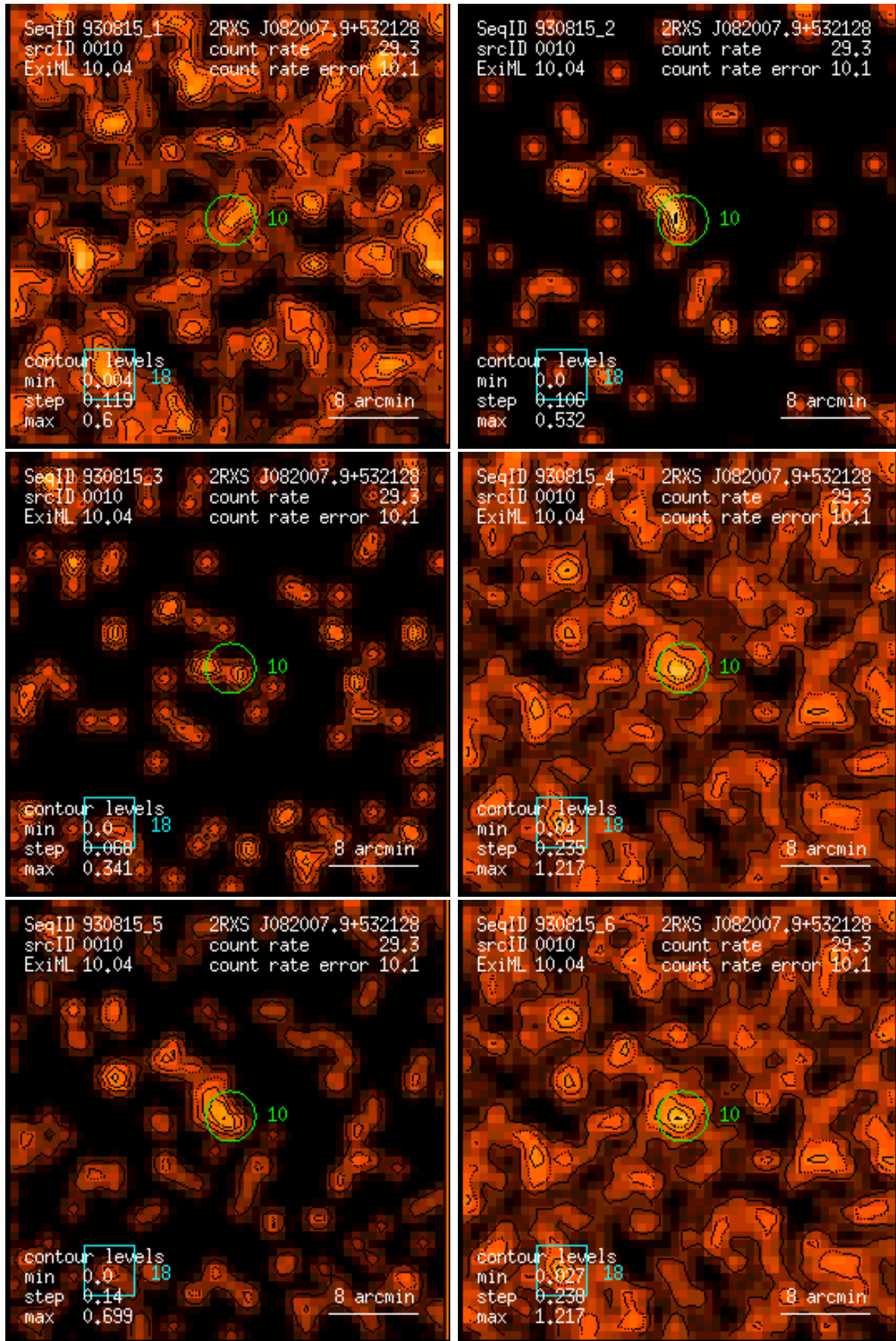
Figure 10: RASS 930815: detection 0010: band rate images, Gaussian filter: (1) PSPC channels 11 – 41, (2) 52 – 90, (3) 91 – 201, (4) 11 – 235, (5) 52 – 201, (6) 11 – 201. Broad band rates in counts/ks. Band rate contour levels in counts/ks/arcmin 2 .
