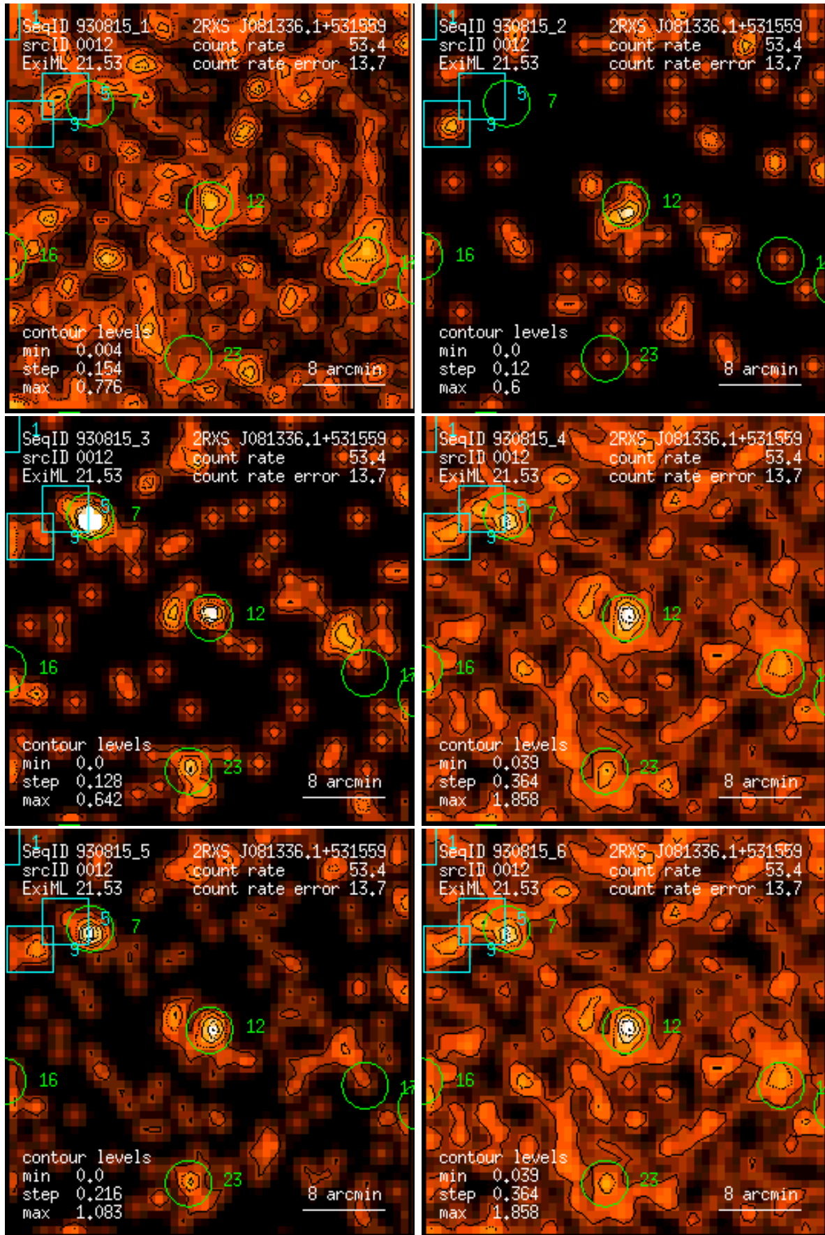
Figure 12: RASS 930815: detection 0012: band rate images, Gaussian filter: (1) PSPC channels 11 – 41, (2) 52 – 90, (3) 91 – 201, (4) 11 – 235, (5) 52 – 201, (6) 11 – 201. Broad band rates in counts/ks. Band rate contour levels in counts/ks/arcmin 2 .
