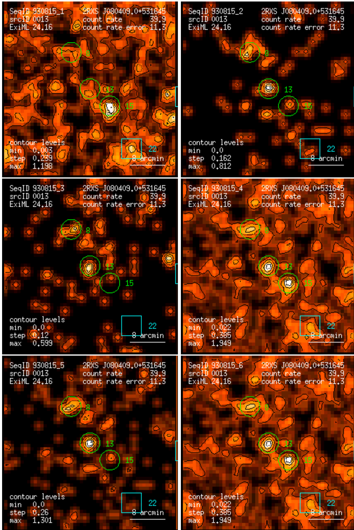
Figure 13: RASS 930815: detection 0013: band rate images, Gaussian filter: (1) PSPC channels 11 – 41, (2) 52 – 90, (3) 91 – 201, (4) 11 – 235, (5) 52 – 201, (6) 11 – 201. Broad band rates in counts/ks. Band rate contour levels in counts/ks/arcmin 2 .
