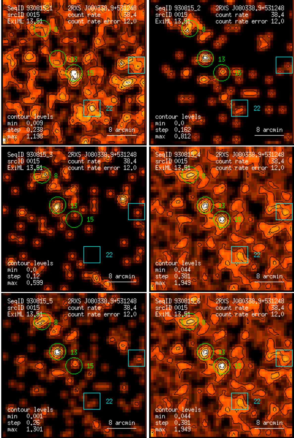
Figure 15: RASS 930815: detection 0015: band rate images, Gaussian filter: (1) PSPC channels 11 – 41, (2) 52 – 90, (3) 91 – 201, (4) 11 – 235, (5) 52 – 201, (6) 11 – 201. Broad band rates in counts/ks. Band rate contour levels in counts/ks/arcmin 2 .
