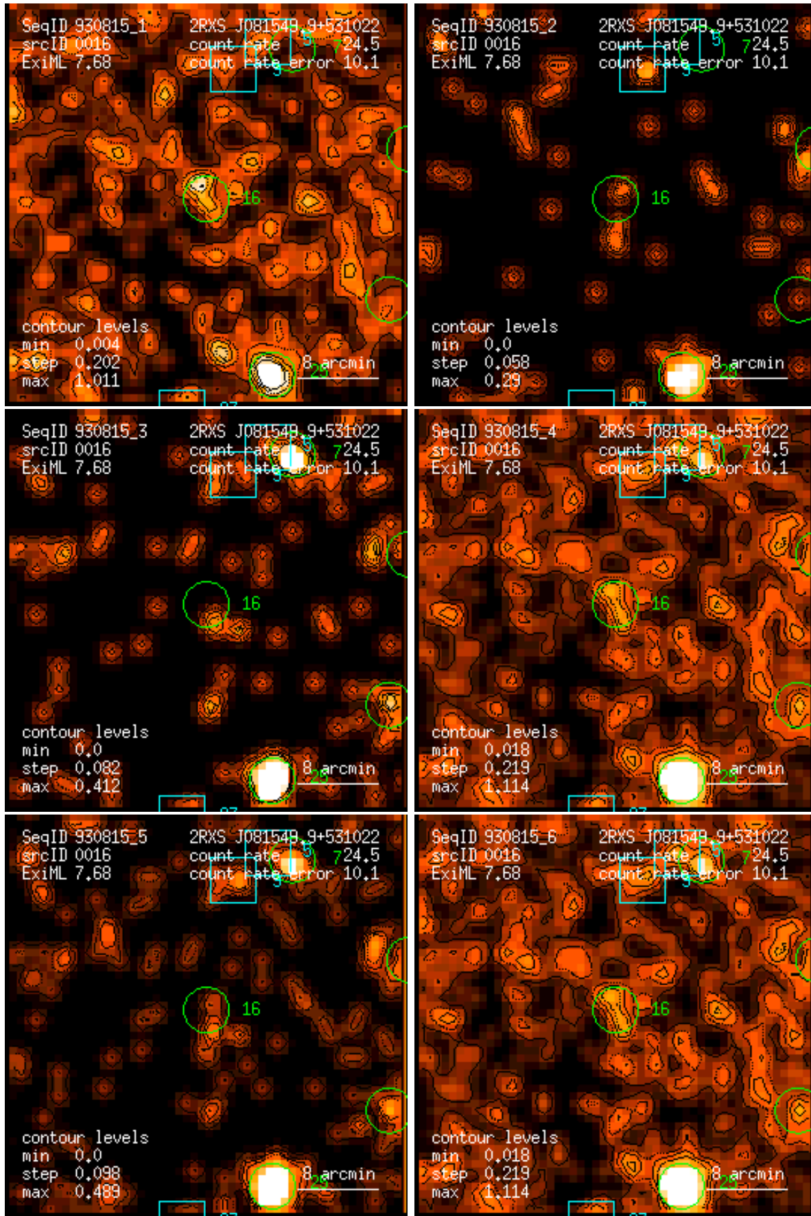
Figure 16: RASS 930815: detection 0016: band rate images, Gaussian filter: (1) PSPC channels 11 – 41, (2) 52 – 90, (3) 91 – 201, (4) 11 – 235, (5) 52 – 201, (6) 11 – 201. Broad band rates in counts/ks. Band rate contour levels in counts/ks/arcmin 2 .
