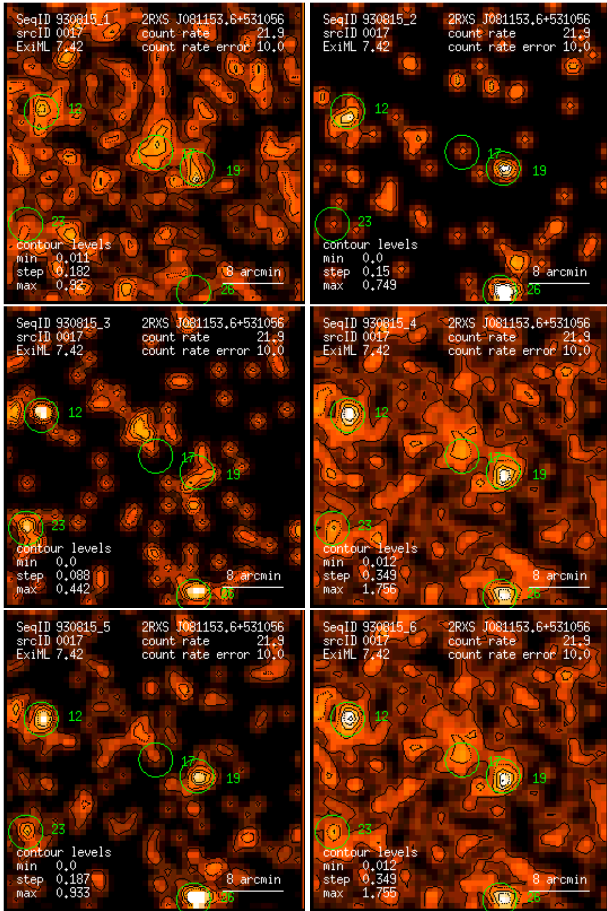
Figure 17: RASS 930815: detection 0017: band rate images, Gaussian filter: (1) PSPC channels 11 – 41, (2) 52 – 90, (3) 91 – 201, (4) 11 – 235, (5) 52 – 201, (6) 11 – 201. Broad band rates in counts/ks. Band rate contour levels in counts/ks/arcmin 2 .
