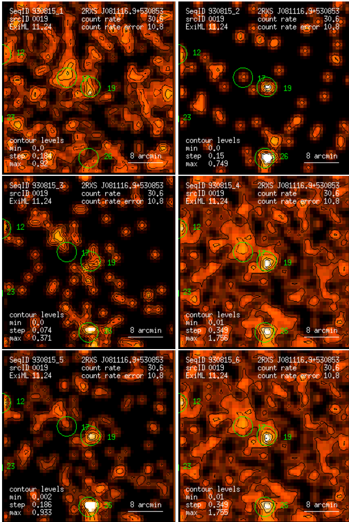
Figure 19: RASS 930815: detection 0019: band rate images, Gaussian filter: (1) PSPC channels 11 – 41, (2) 52 – 90, (3) 91 – 201, (4) 11 – 235, (5) 52 – 201, (6) 11 – 201. Broad band rates in counts/ks. Band rate contour levels in counts/ks/arcmin 2 .
