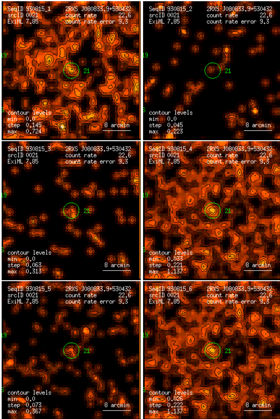
Figure 21: RASS 930815: detection 0021: band rate images, Gaussian filter: (1) PSPC channels 11 – 41, (2) 52 – 90, (3) 91 – 201, (4) 11 – 235, (5) 52 – 201, (6) 11 – 201. Broad band rates in counts/ks. Band rate contour levels in counts/ks/arcmin 2 .
