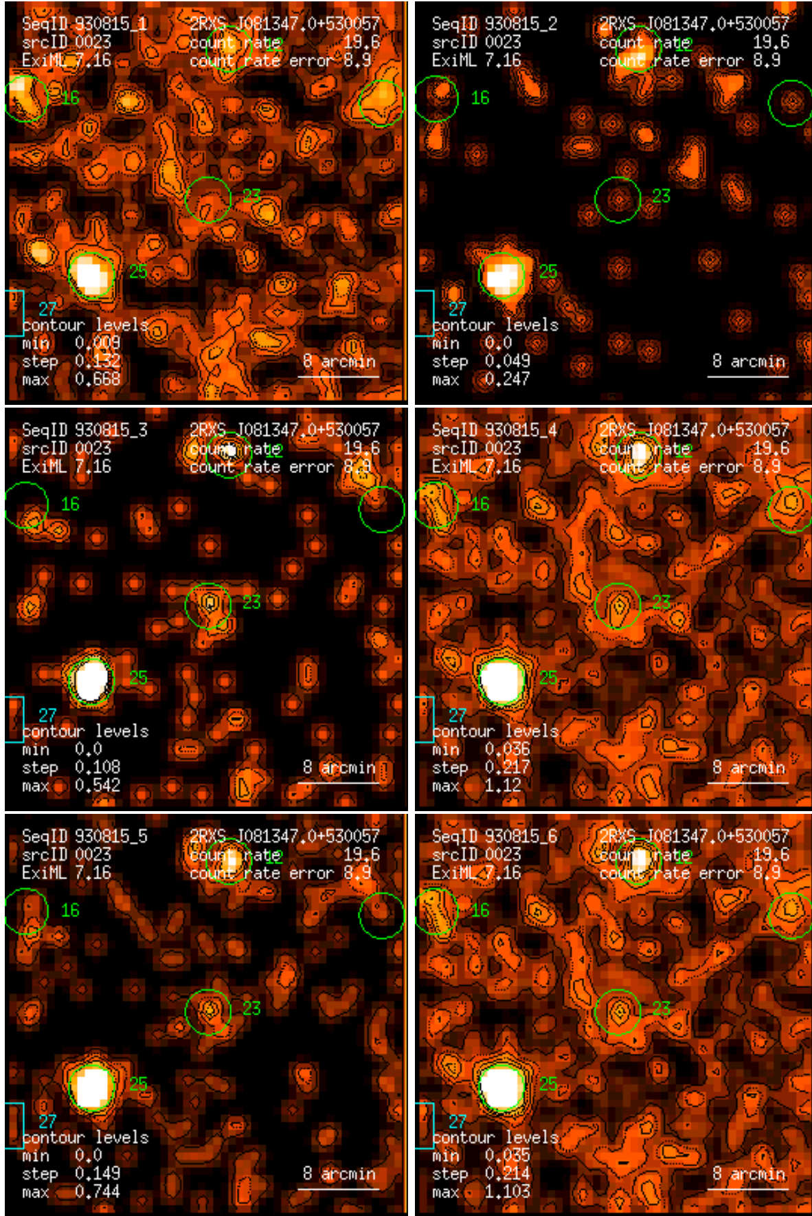
Figure 23: RASS 930815: detection 0023: band rate images, Gaussian filter: (1) PSPC channels 11 – 41, (2) 52 – 90, (3) 91 – 201, (4) 11 – 235, (5) 52 – 201, (6) 11 – 201. Broad band rates in counts/ks. Band rate contour levels in counts/ks/arcmin 2 .
