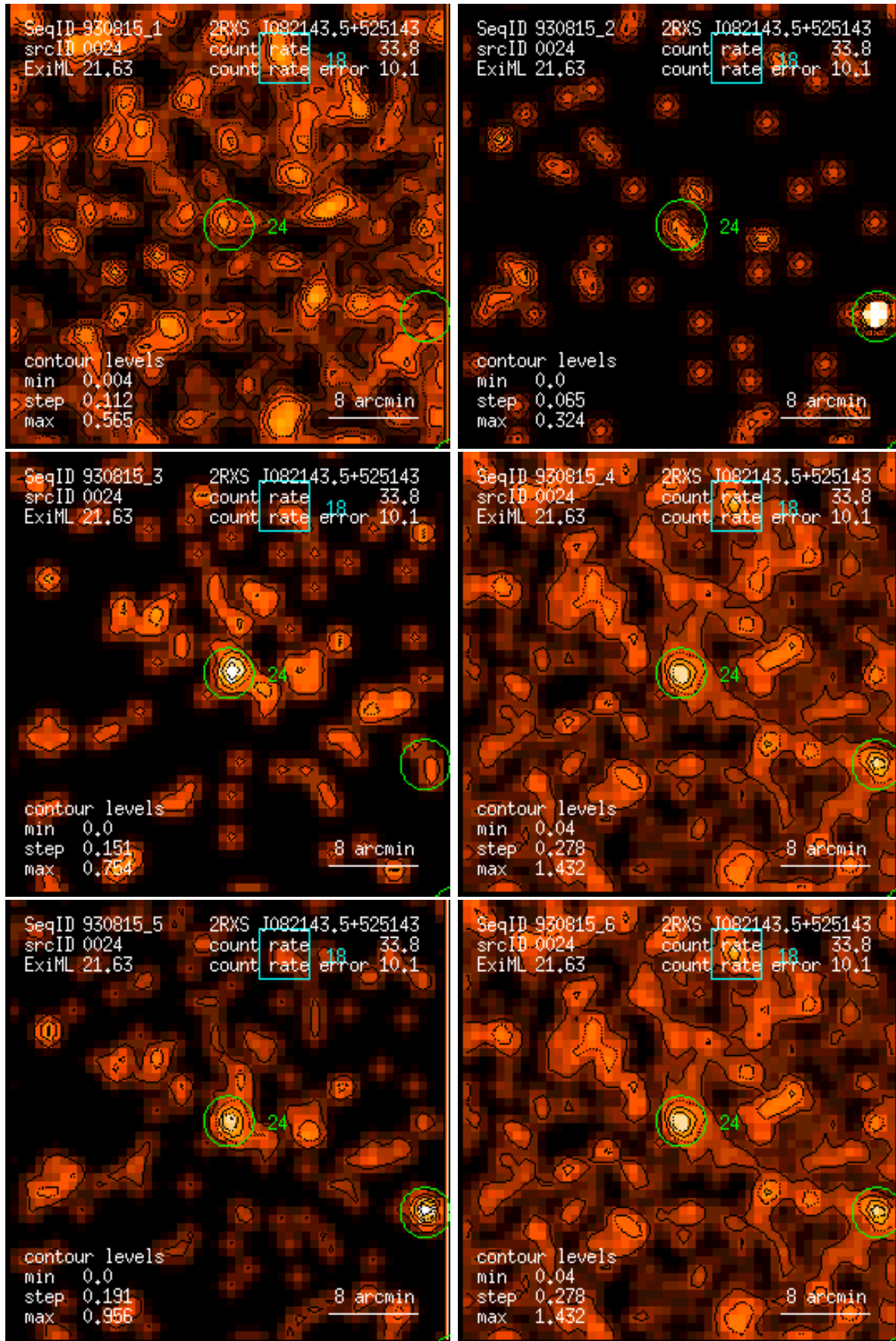
Figure 24: RASS 930815: detection 0024: band rate images, Gaussian filter: (1) PSPC channels 11 – 41, (2) 52 – 90, (3) 91 – 201, (4) 11 – 235, (5) 52 – 201, (6) 11 – 201. Broad band rates in counts/ks. Band rate contour levels in counts/ks/arcmin 2 .
