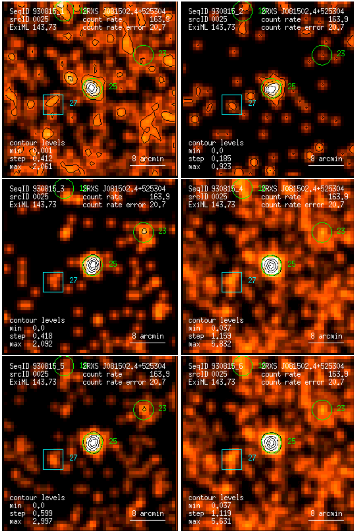
Figure 25: RASS 930815: detection 0025: band rate images, Gaussian filter: (1) PSPC channels 11 – 41, (2) 52 – 90, (3) 91 – 201, (4) 11 – 235, (5) 52 – 201, (6) 11 – 201. Broad band rates in counts/ks. Band rate contour levels in counts/ks/arcmin 2 .
