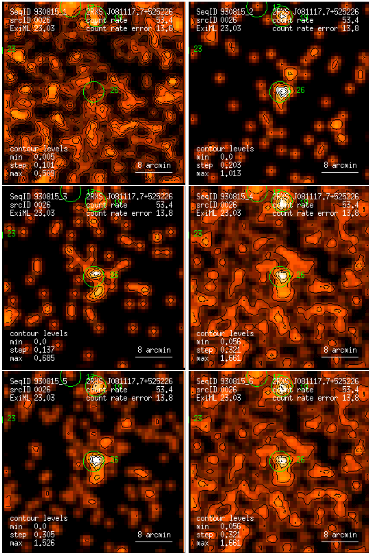
Figure 26: RASS 930815: detection 0026: band rate images, Gaussian filter: (1) PSPC channels 11 – 41, (2) 52 – 90, (3) 91 – 201, (4) 11 – 235, (5) 52 – 201, (6) 11 – 201. Broad band rates in counts/ks. Band rate contour levels in counts/ks/arcmin 2 .
