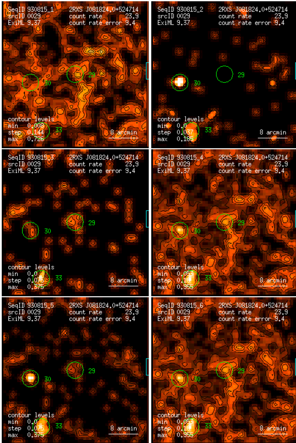
Figure 29: RASS 930815: detection 0029: band rate images, Gaussian filter: (1) PSPC channels 11 – 41, (2) 52 – 90, (3) 91 – 201, (4) 11 – 235, (5) 52 – 201, (6) 11 – 201. Broad band rates in counts/ks. Band rate contour levels in counts/ks/arcmin 2 .
