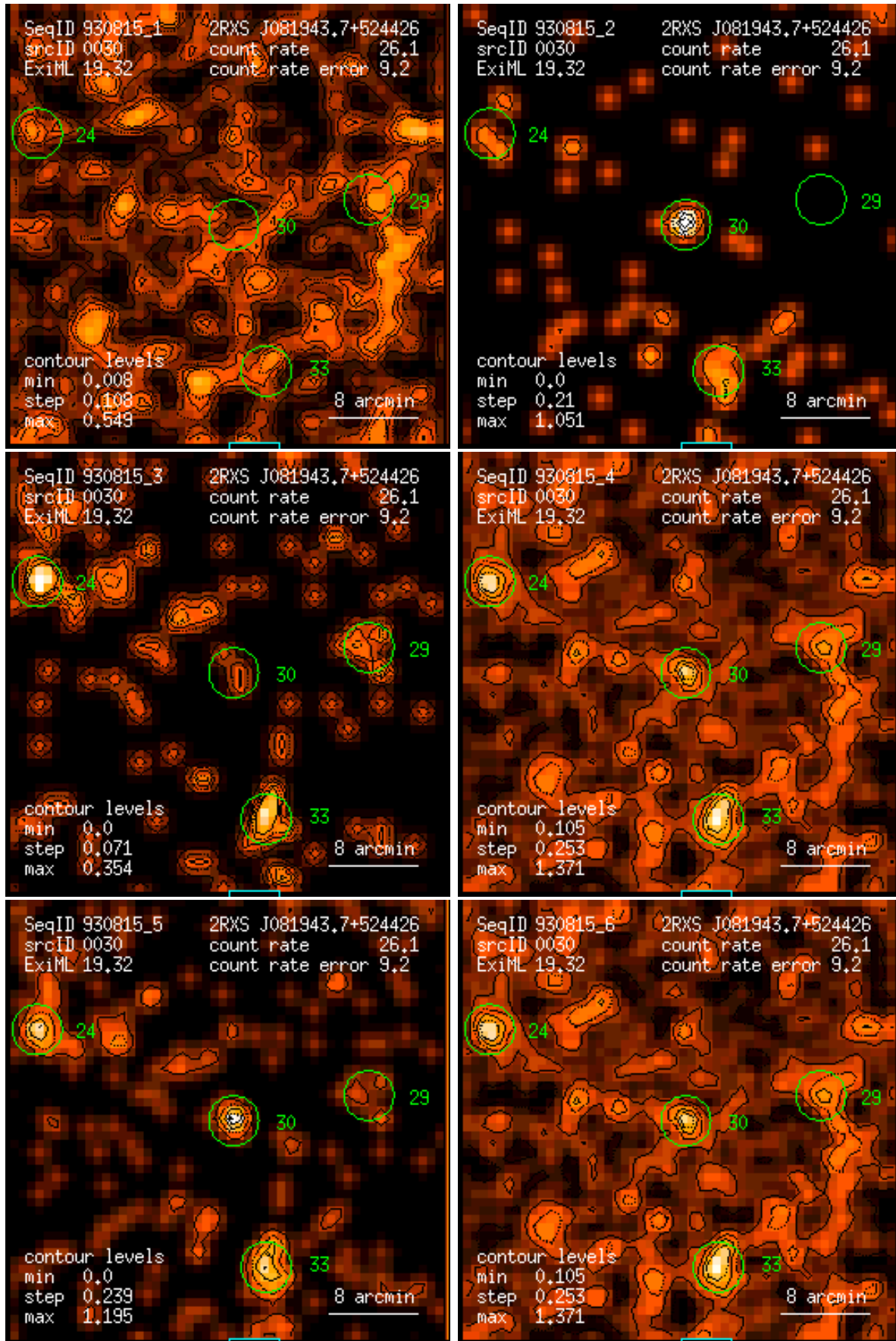
Figure 30: RASS 930815: detection 0030: band rate images, Gaussian filter: (1) PSPC channels 11 – 41, (2) 52 – 90, (3) 91 – 201, (4) 11 – 235, (5) 52 – 201, (6) 11 – 201. Broad band rates in counts/ks. Band rate contour levels in counts/ks/arcmin 2 .
