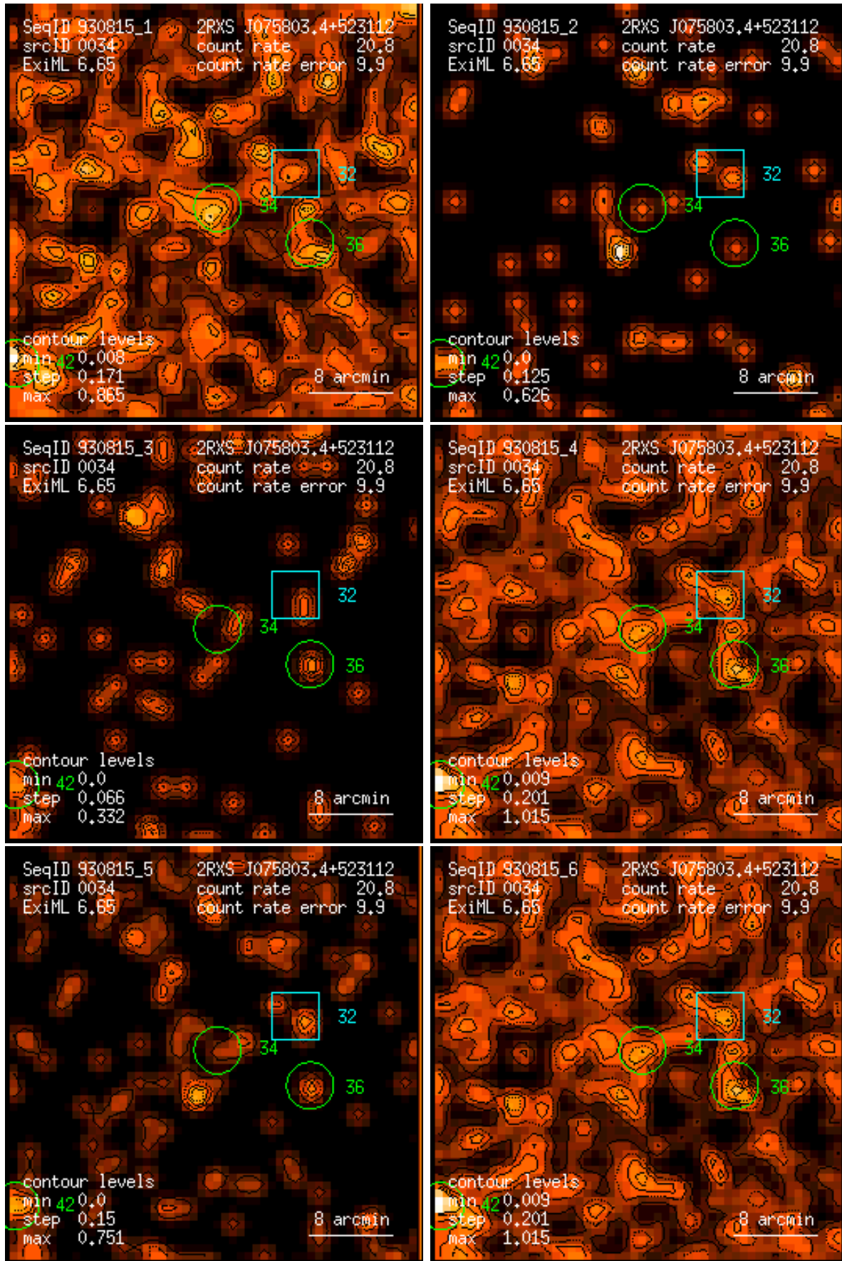
Figure 34: RASS 930815: detection 0034: band rate images, Gaussian filter: (1) PSPC channels 11 – 41, (2) 52 – 90, (3) 91 – 201, (4) 11 – 235, (5) 52 – 201, (6) 11 – 201. Broad band rates in counts/ks. Band rate contour levels in counts/ks/arcmin 2 .
