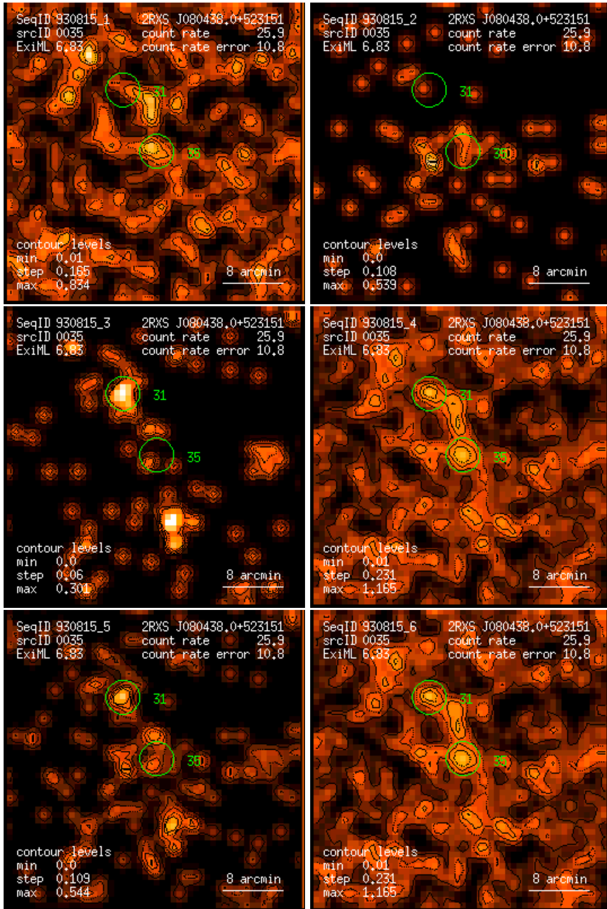
Figure 35: RASS 930815: detection 0035: band rate images, Gaussian filter: (1) PSPC channels 11 – 41, (2) 52 – 90, (3) 91 – 201, (4) 11 – 235, (5) 52 – 201, (6) 11 – 201. Broad band rates in counts/ks. Band rate contour levels in counts/ks/arcmin 2 .
