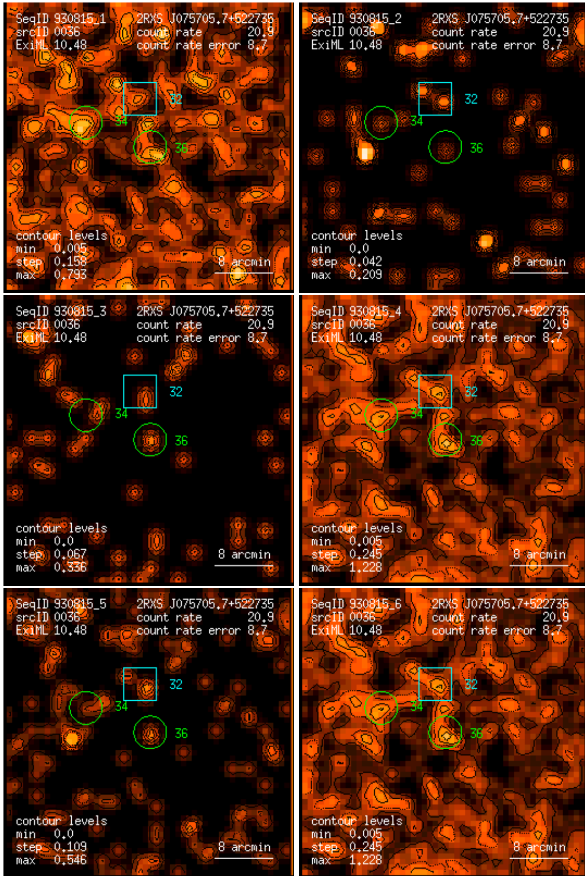
Figure 36: RASS 930815: detection 0036: band rate images, Gaussian filter: (1) PSPC channels 11 – 41, (2) 52 – 90, (3) 91 – 201, (4) 11 – 235, (5) 52 – 201, (6) 11 – 201. Broad band rates in counts/ks. Band rate contour levels in counts/ks/arcmin 2 .
