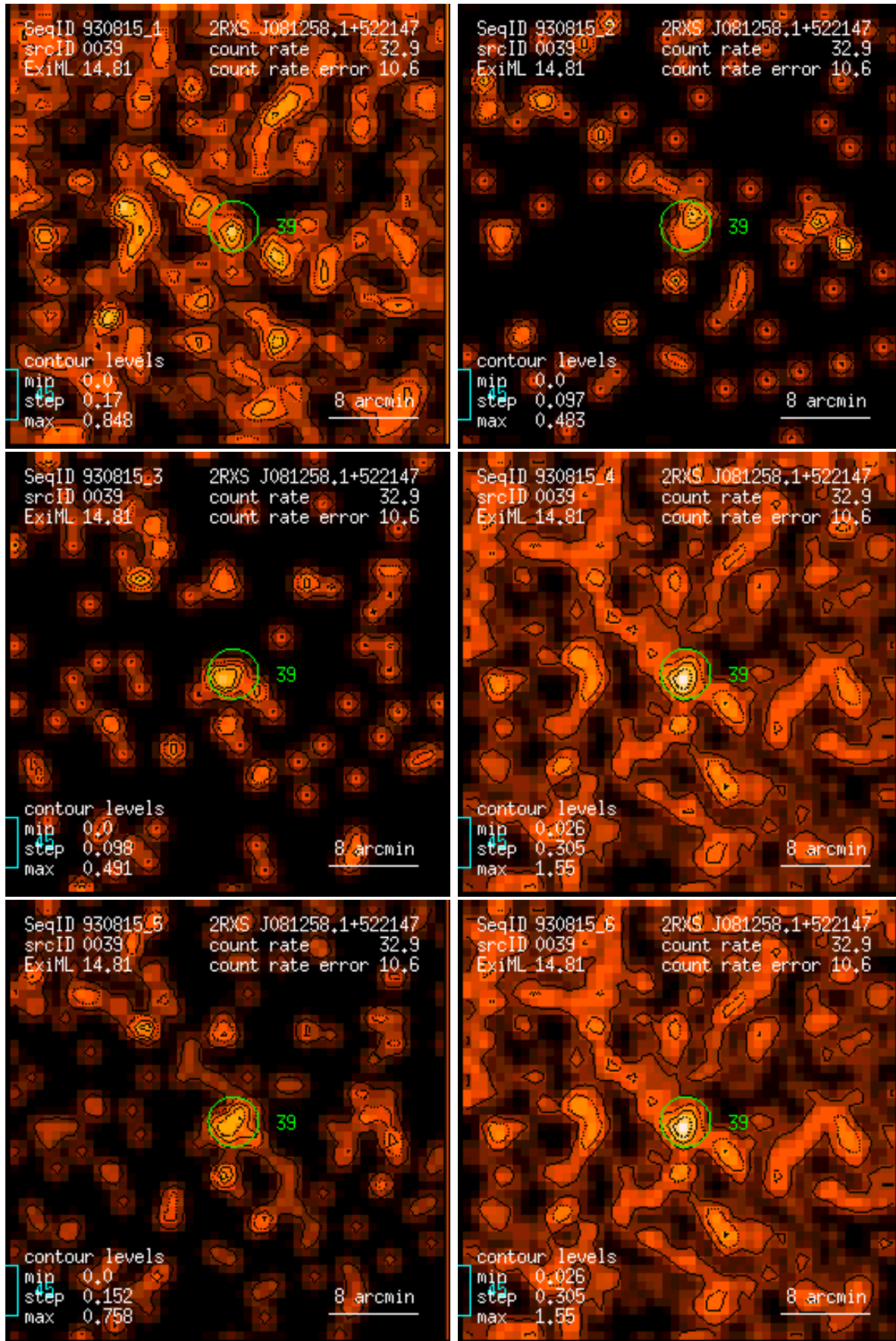
Figure 39: RASS 930815: detection 0039: band rate images, Gaussian filter: (1) PSPC channels 11 – 41, (2) 52 – 90, (3) 91 – 201, (4) 11 – 235, (5) 52 – 201, (6) 11 – 201. Broad band rates in counts/ks. Band rate contour levels in counts/ks/arcmin 2 .
