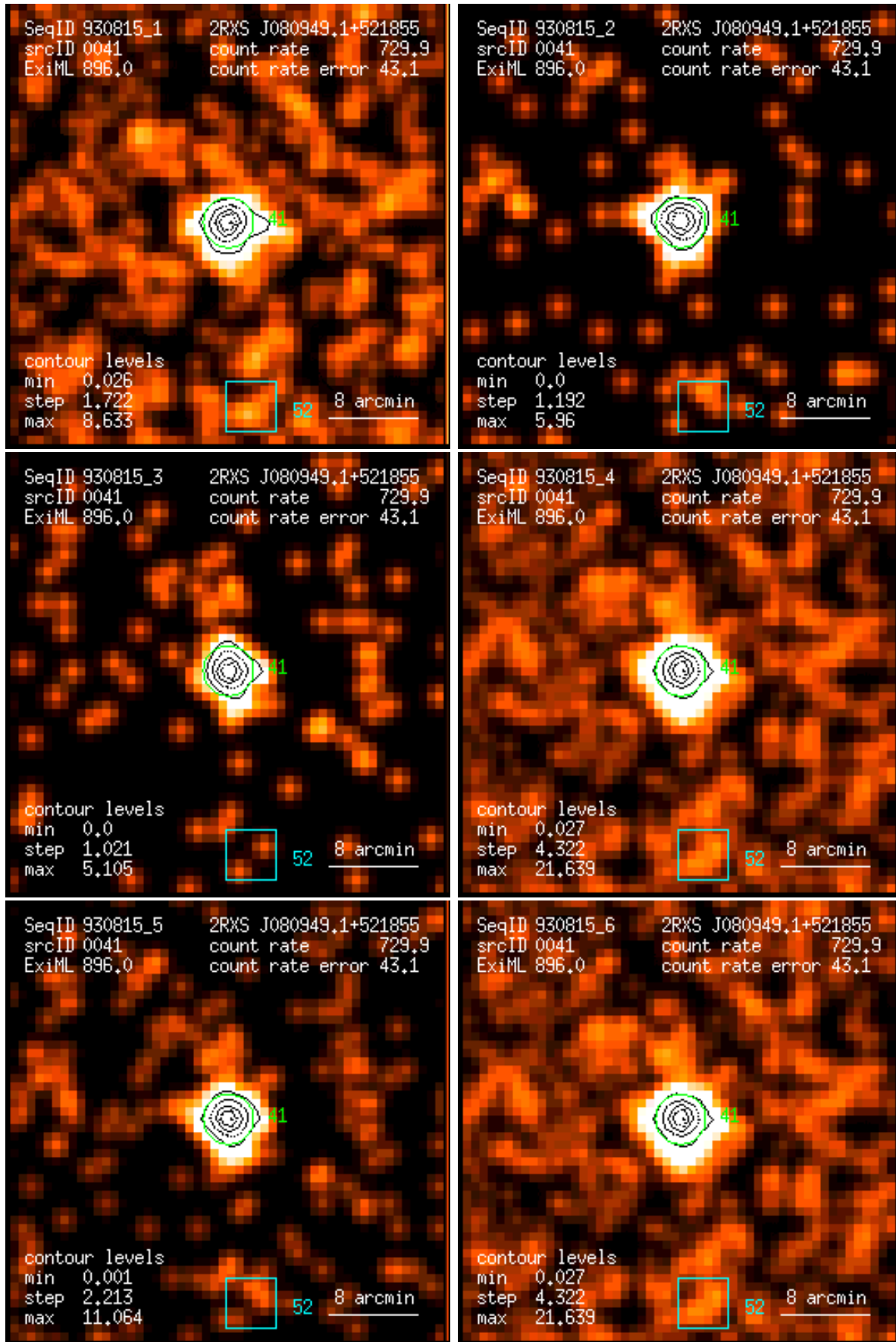
Figure 41: RASS 930815: detection 0041: band rate images, Gaussian filter: (1) PSPC channels 11 – 41, (2) 52 – 90, (3) 91 – 201, (4) 11 – 235, (5) 52 – 201, (6) 11 – 201. Broad band rates in counts/ks. Band rate contour levels in counts/ks/arcmin 2 .
