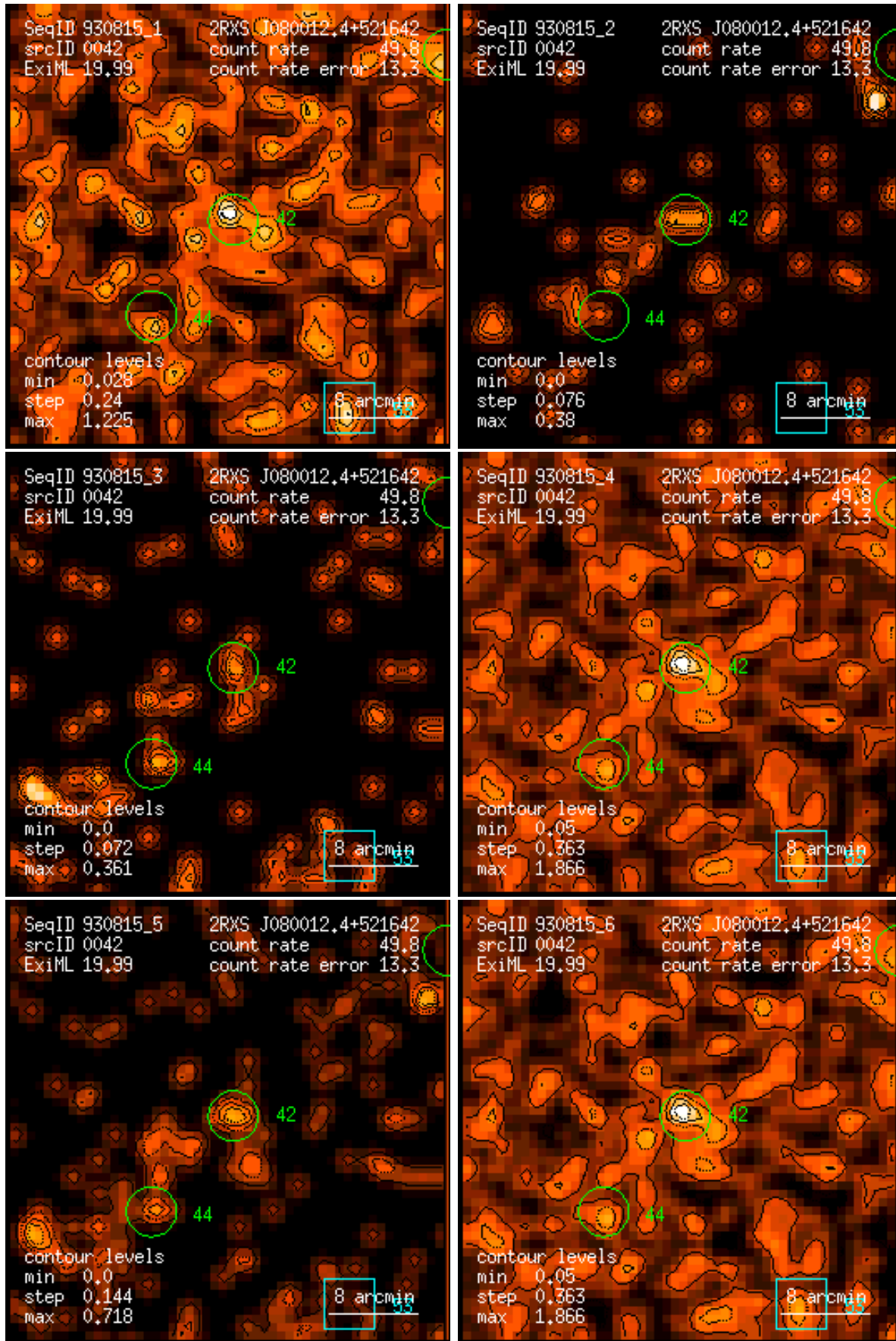
Figure 42: RASS 930815: detection 0042: band rate images, Gaussian filter: (1) PSPC channels 11 – 41, (2) 52 – 90, (3) 91 – 201, (4) 11 – 235, (5) 52 – 201, (6) 11 – 201. Broad band rates in counts/ks. Band rate contour levels in counts/ks/arcmin 2 .
