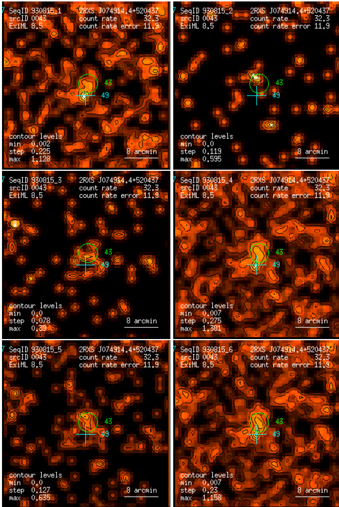
Figure 43: RASS 930815: detection 0043: band rate images, Gaussian filter: (1) PSPC channels 11 – 41, (2) 52 – 90, (3) 91 – 201, (4) 11 – 235, (5) 52 – 201, (6) 11 – 201. Broad band rates in counts/ks. Band rate contour levels in counts/ks/arcmin 2 .
