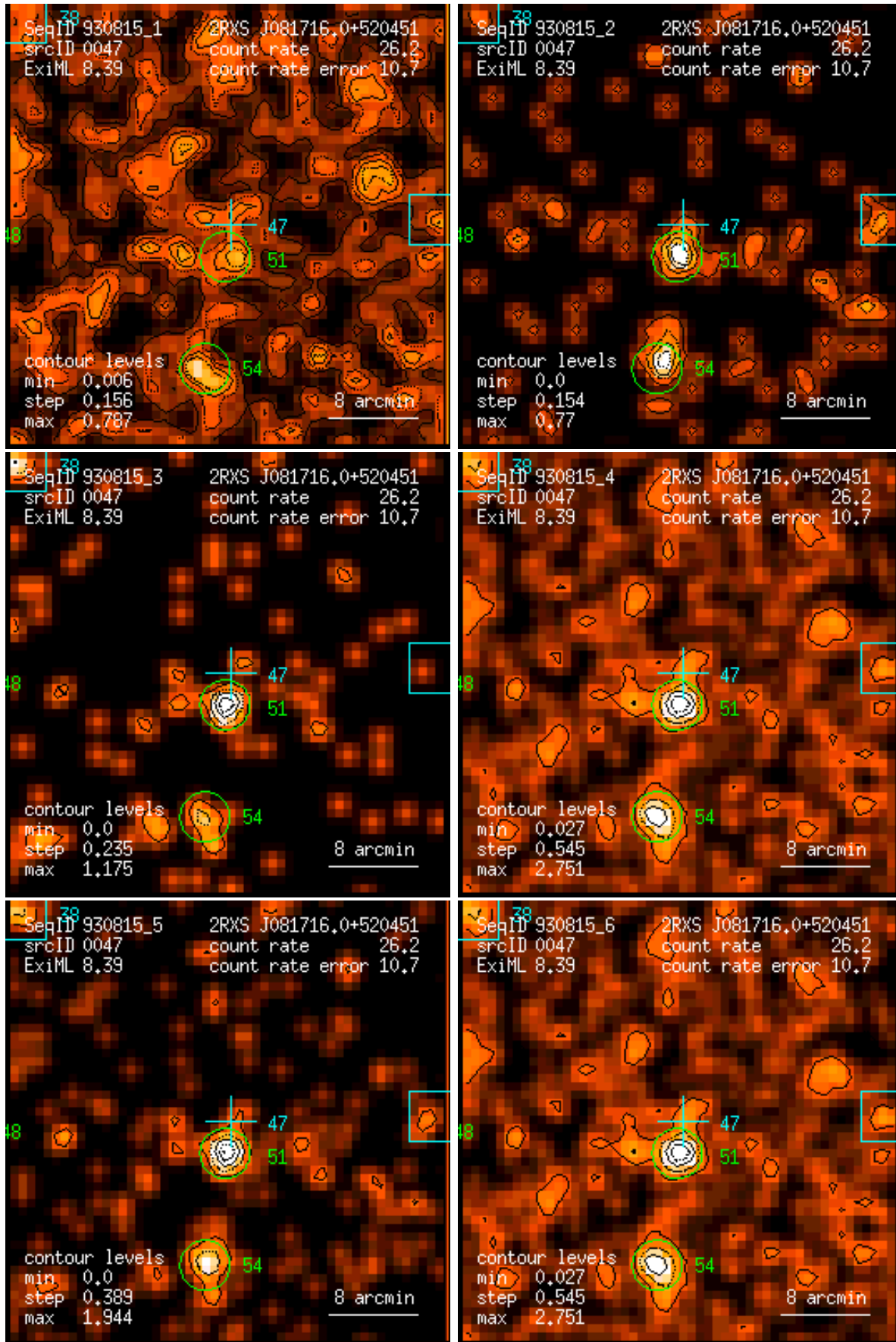
Figure 47: RASS 930815: detection 0047: band rate images, Gaussian filter: (1) PSPC channels 11 – 41, (2) 52 – 90, (3) 91 – 201, (4) 11 – 235, (5) 52 – 201, (6) 11 – 201. Broad band rates in counts/ks. Band rate contour levels in counts/ks/arcmin 2 .
