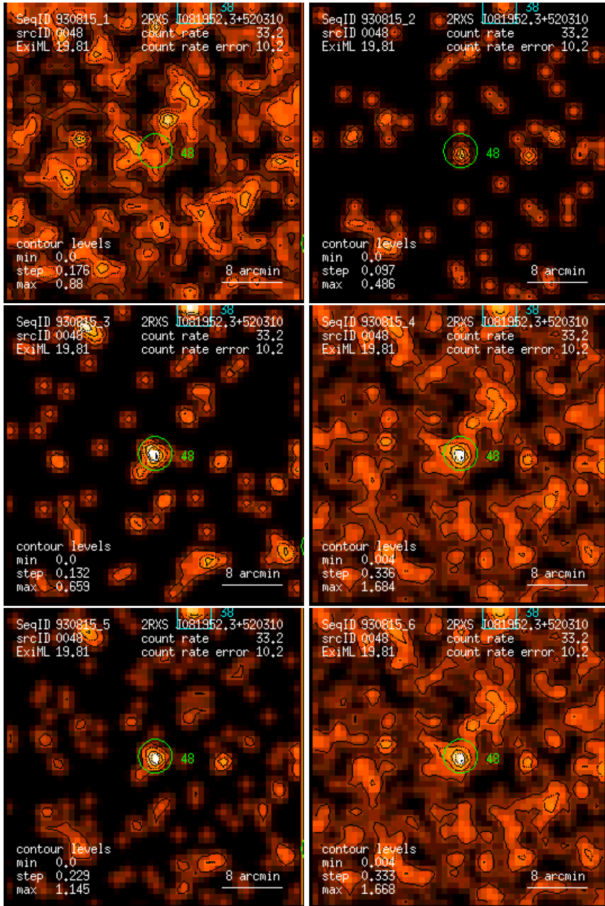
Figure 48: RASS 930815: detection 0048: band rate images, Gaussian filter: (1) PSPC channels 11 – 41, (2) 52 – 90, (3) 91 – 201, (4) 11 – 235, (5) 52 – 201, (6) 11 – 201. Broad band rates in counts/ks. Band rate contour levels in counts/ks/arcmin 2 .
