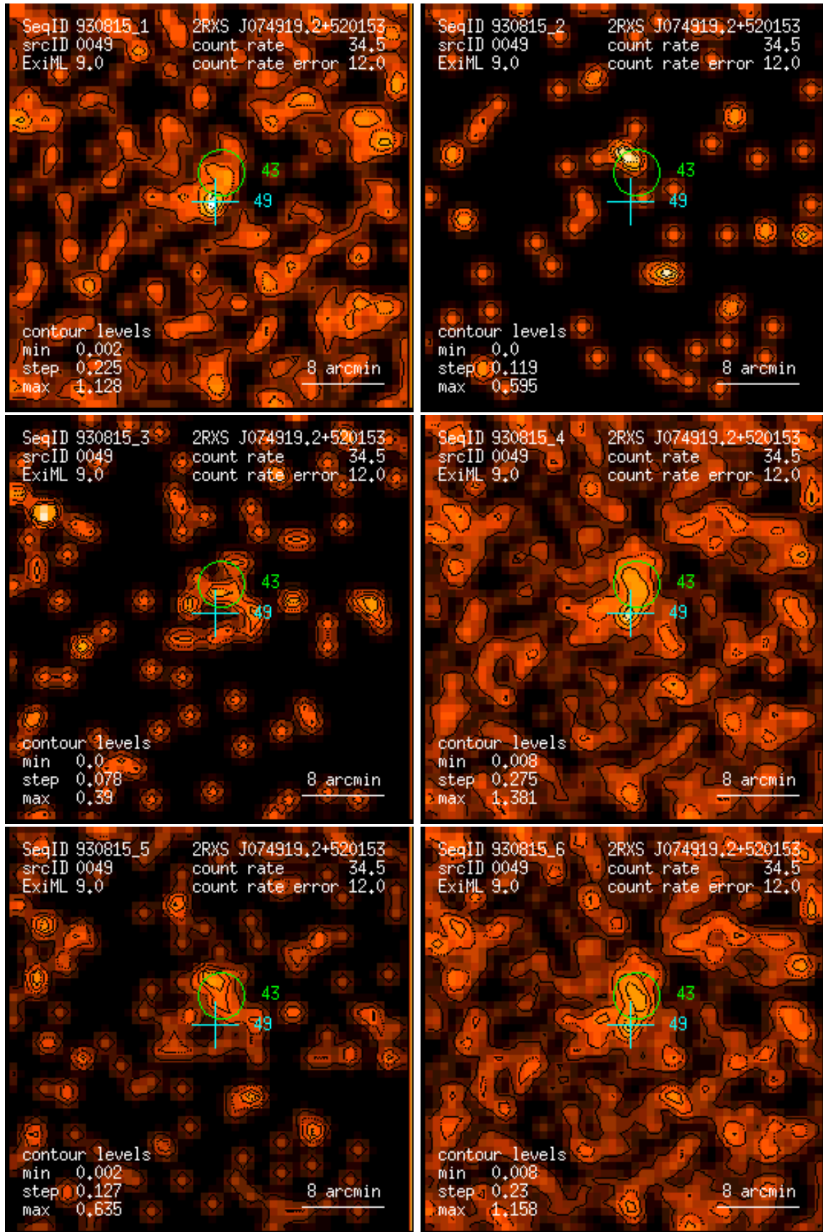
Figure 49: RASS 930815: detection 0049: band rate images, Gaussian filter: (1) PSPC channels 11 – 41, (2) 52 – 90, (3) 91 – 201, (4) 11 – 235, (5) 52 – 201, (6) 11 – 201. Broad band rates in counts/ks. Band rate contour levels in counts/ks/arcmin 2 .
