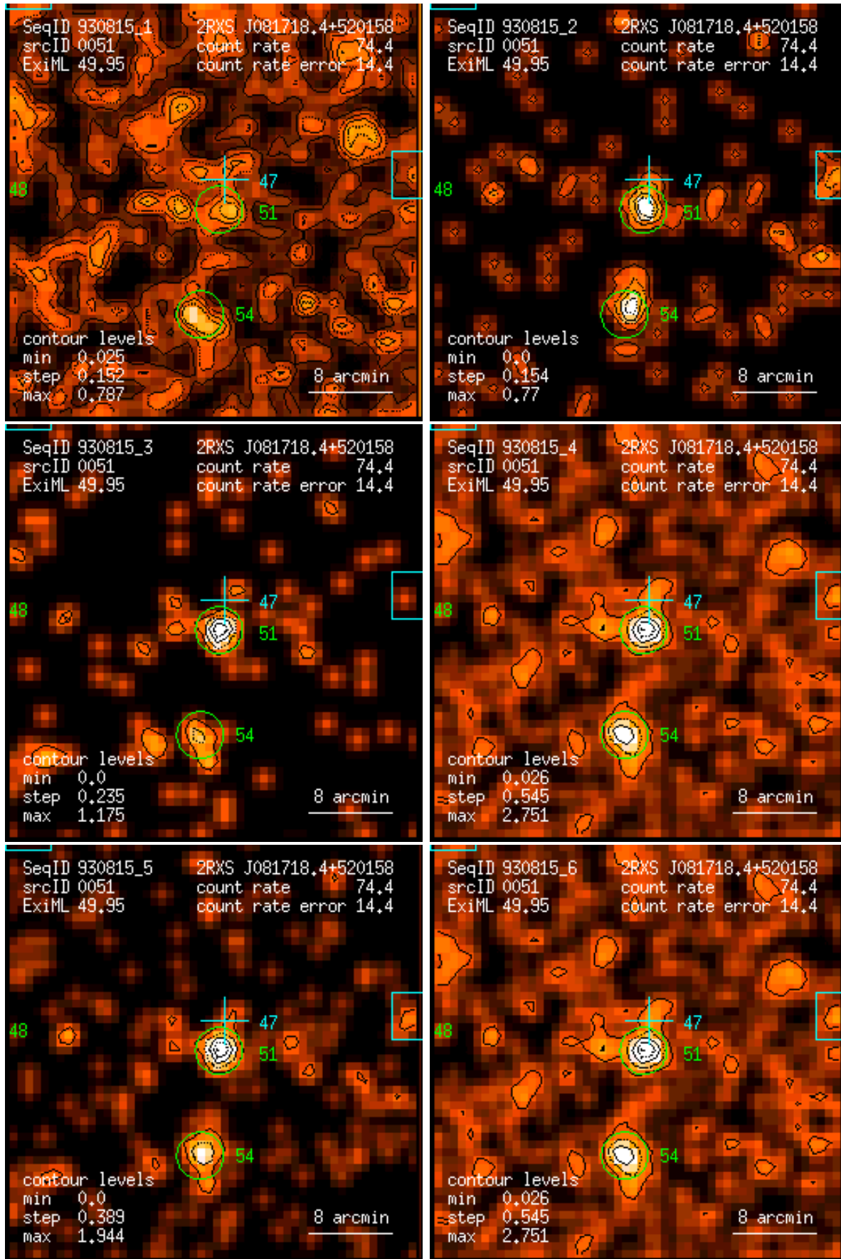
Figure 51: RASS 930815: detection 0051: band rate images, Gaussian filter: (1) PSPC channels 11 – 41, (2) 52 – 90, (3) 91 – 201, (4) 11 – 235, (5) 52 – 201, (6) 11 – 201. Broad band rates in counts/ks. Band rate contour levels in counts/ks/arcmin 2 .
