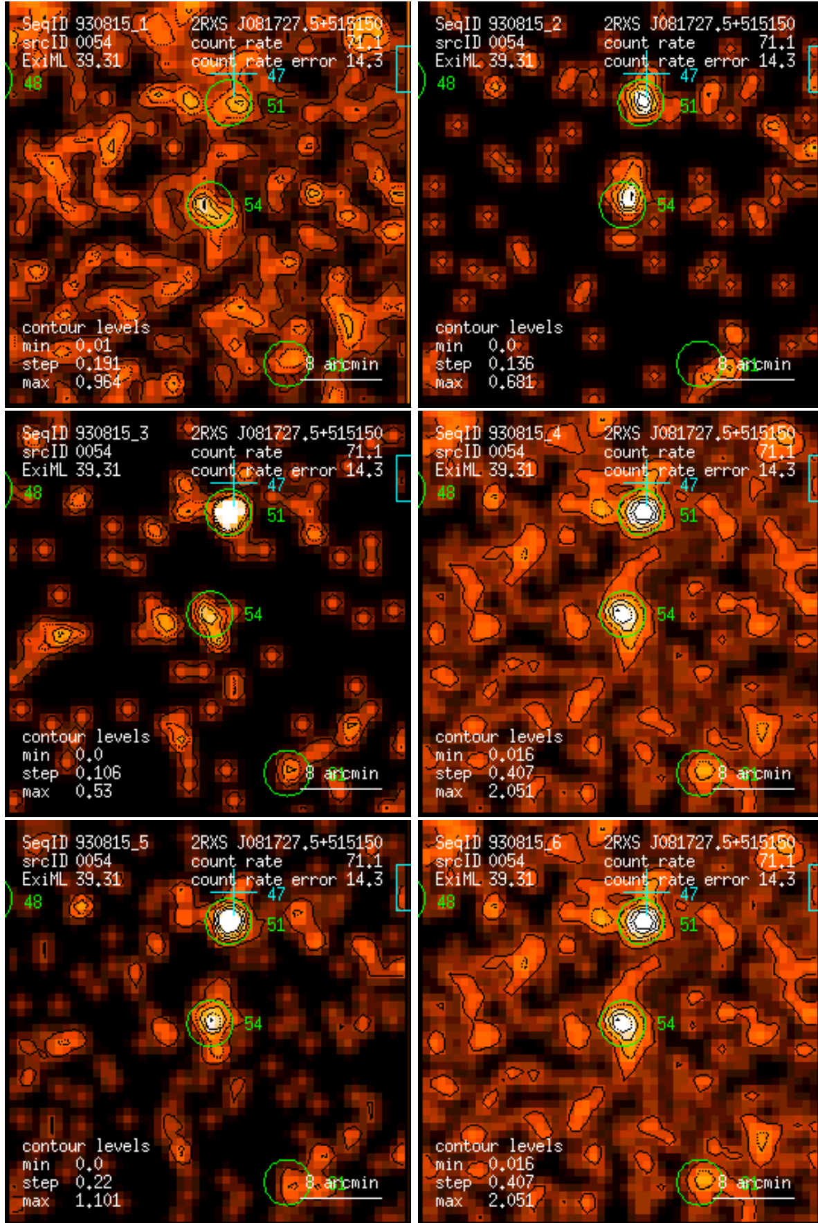
Figure 54: RASS 930815: detection 0054: band rate images, Gaussian filter: (1) PSPC channels 11 – 41, (2) 52 – 90, (3) 91 – 201, (4) 11 – 235, (5) 52 – 201, (6) 11 – 201. Broad band rates in counts/ks. Band rate contour levels in counts/ks/arcmin 2 .
