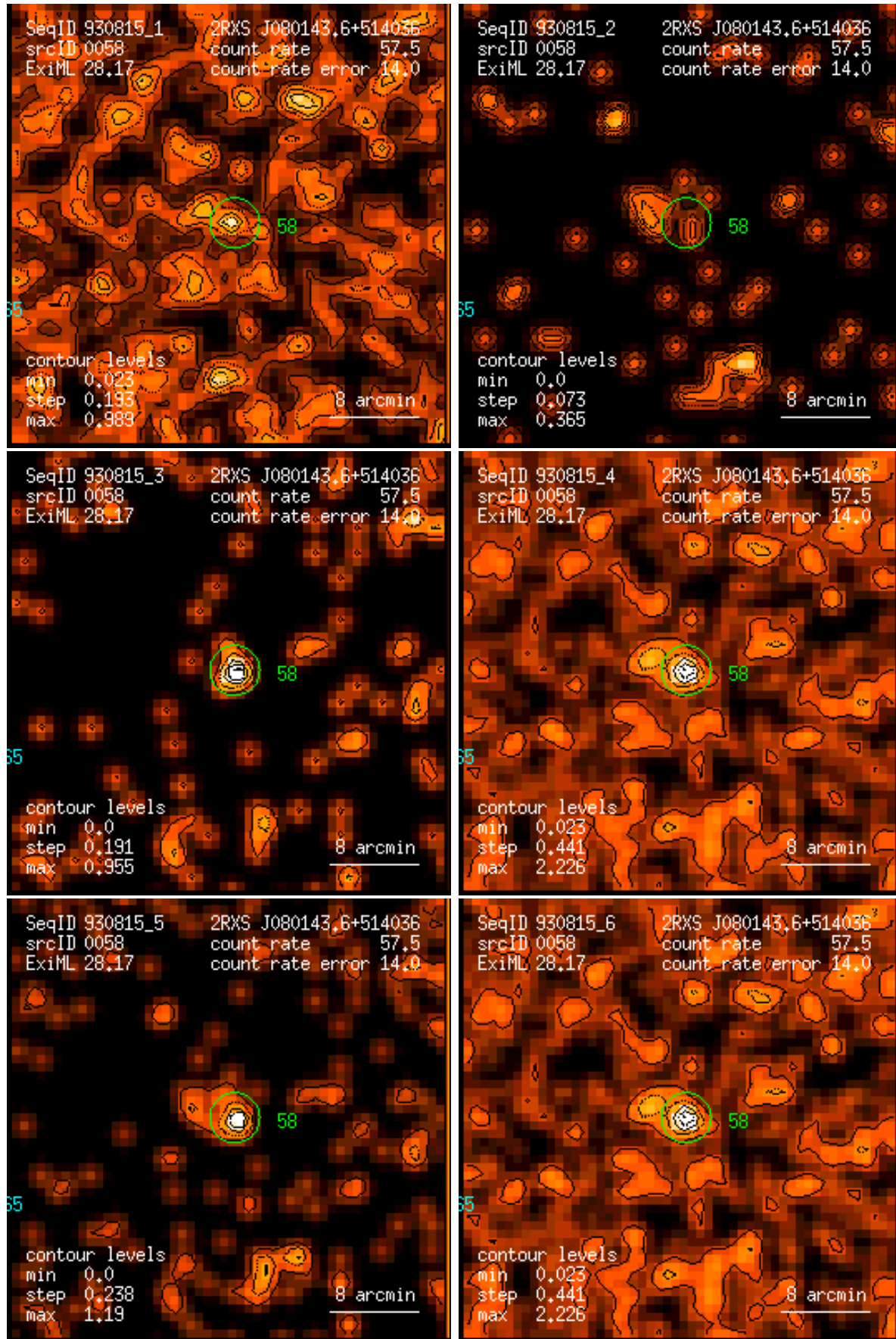
Figure 58: RASS 930815: detection 0058: band rate images, Gaussian filter: (1) PSPC channels 11 – 41, (2) 52 – 90, (3) 91 – 201, (4) 11 – 235, (5) 52 – 201, (6) 11 – 201. Broad band rates in counts/ks. Band rate contour levels in counts/ks/arcmin 2 .
