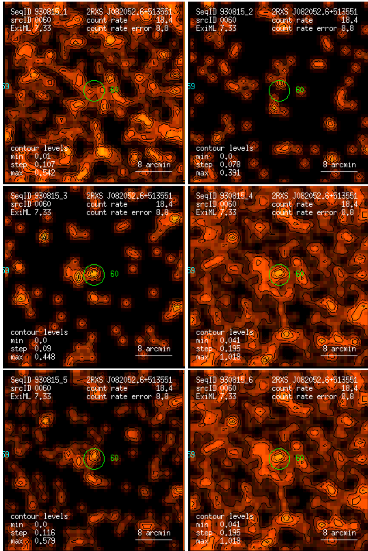
Figure 60: RASS 930815: detection 0060: band rate images, Gaussian filter: (1) PSPC channels 11 – 41, (2) 52 – 90, (3) 91 – 201, (4) 11 – 235, (5) 52 – 201, (6) 11 – 201. Broad band rates in counts/ks. Band rate contour levels in counts/ks/arcmin 2 .
