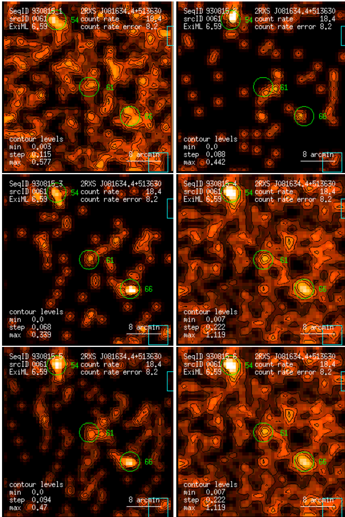
Figure 61: RASS 930815: detection 0061: band rate images, Gaussian filter: (1) PSPC channels 11 – 41, (2) 52 – 90, (3) 91 – 201, (4) 11 – 235, (5) 52 – 201, (6) 11 – 201. Broad band rates in counts/ks. Band rate contour levels in counts/ks/arcmin 2 .
