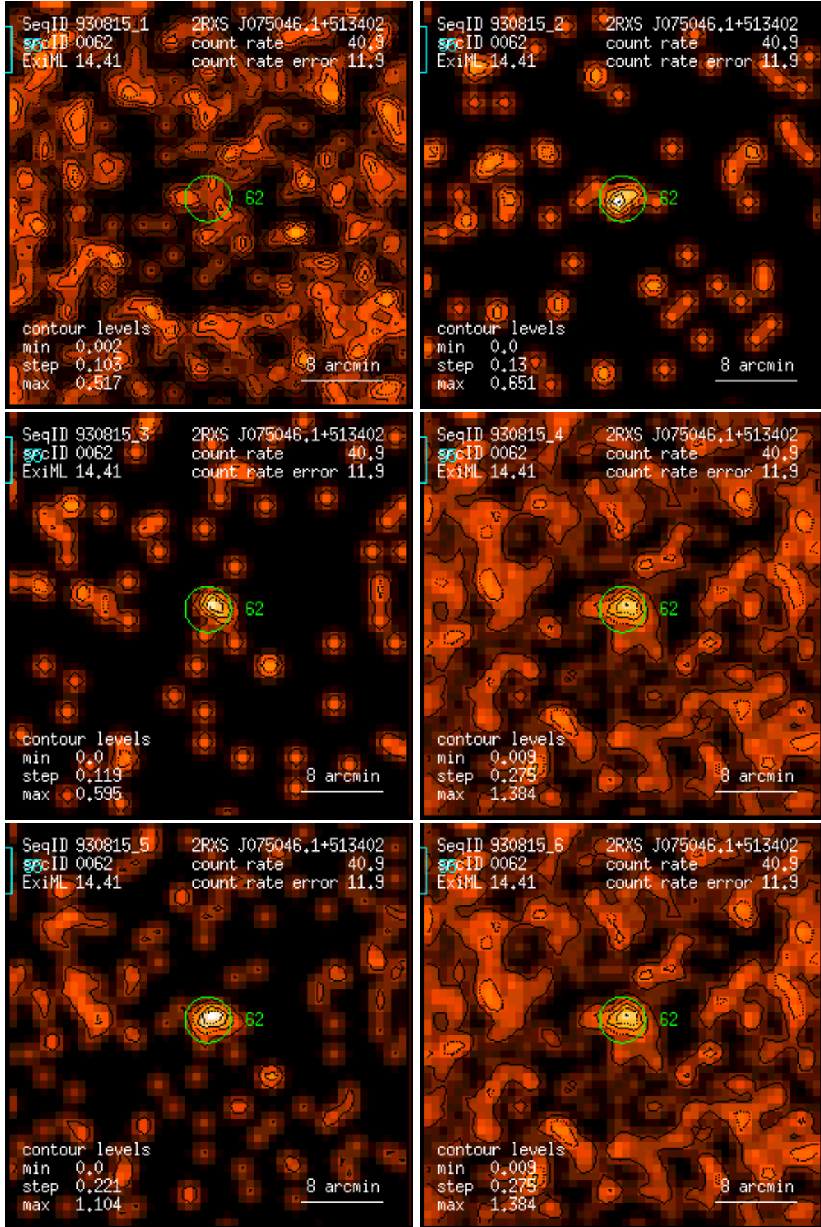
Figure 62: RASS 930815: detection 0062: band rate images, Gaussian filter: (1) PSPC channels 11 – 41, (2) 52 – 90, (3) 91 – 201, (4) 11 – 235, (5) 52 – 201, (6) 11 – 201. Broad band rates in counts/ks. Band rate contour levels in counts/ks/arcmin 2 .
