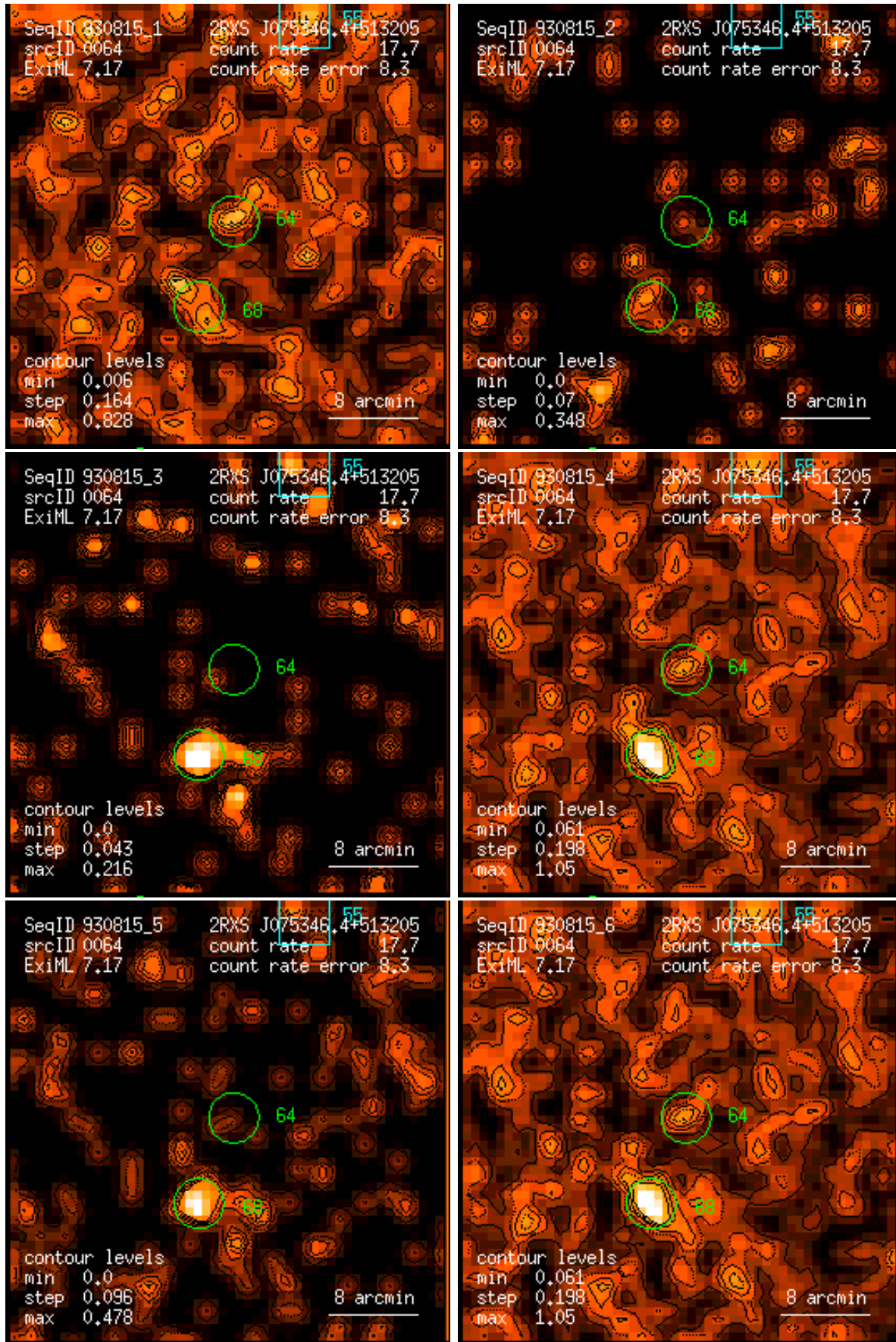
Figure 64: RASS 930815: detection 0064: band rate images, Gaussian filter: (1) PSPC channels 11 – 41, (2) 52 – 90, (3) 91 – 201, (4) 11 – 235, (5) 52 – 201, (6) 11 – 201. Broad band rates in counts/ks. Band rate contour levels in counts/ks/arcmin 2 .
