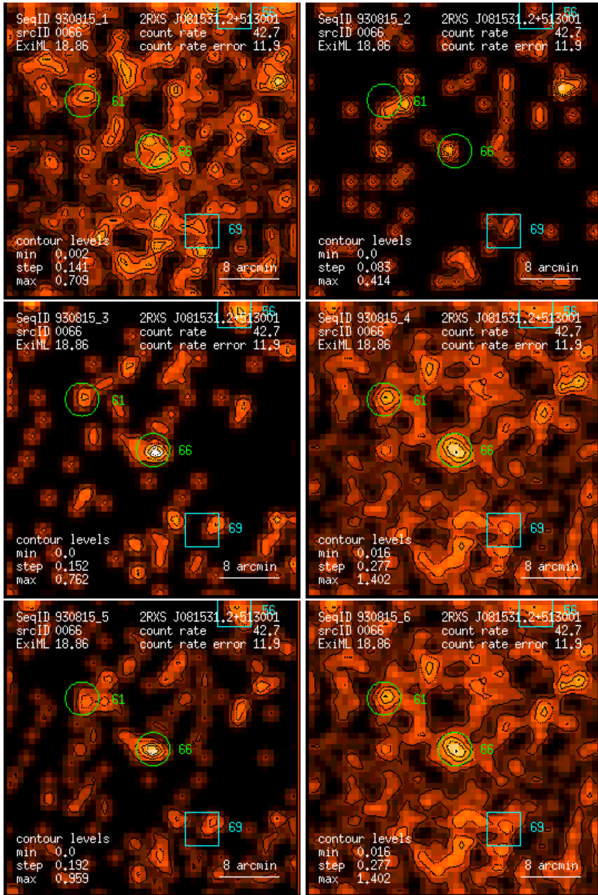
Figure 66: RASS 930815: detection 0066: band rate images, Gaussian filter: (1) PSPC channels 11 – 41, (2) 52 – 90, (3) 91 – 201, (4) 11 – 235, (5) 52 – 201, (6) 11 – 201. Broad band rates in counts/ks. Band rate contour levels in counts/ks/arcmin 2 .
