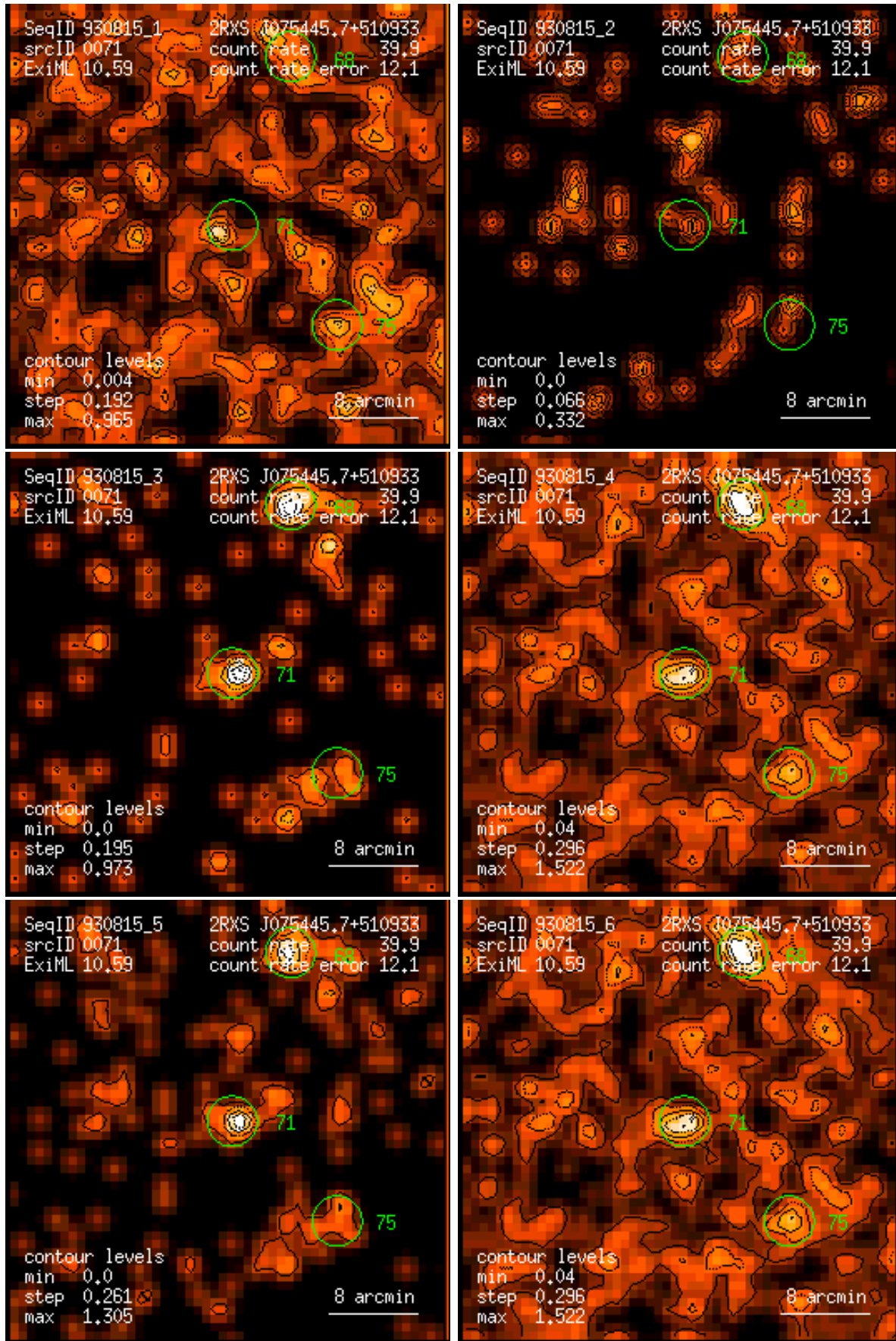
Figure 71: RASS 930815: detection 0071: band rate images, Gaussian filter: (1) PSPC channels 11 – 41, (2) 52 – 90, (3) 91 – 201, (4) 11 – 235, (5) 52 – 201, (6) 11 – 201. Broad band rates in counts/ks. Band rate contour levels in counts/ks/arcmin 2 .
